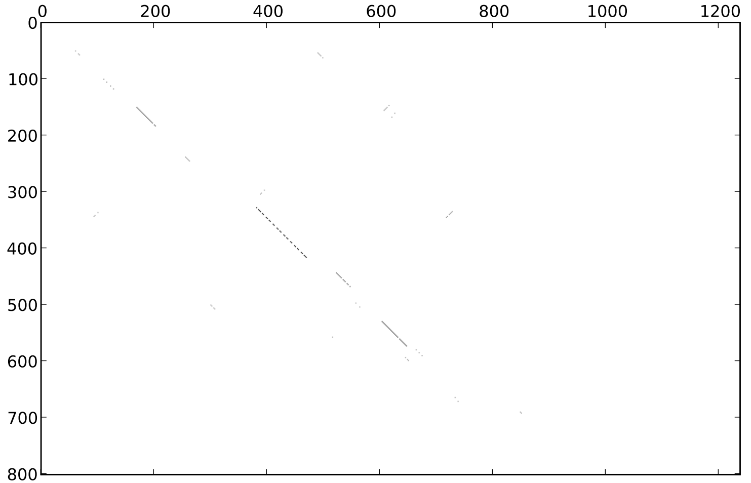
st46_dmel_dvir_blastplot_9_rev_normed
