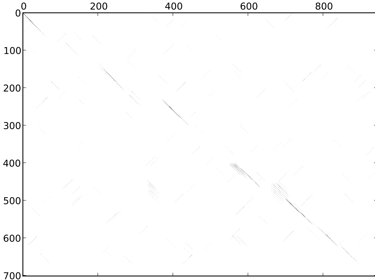
st2_dmel_dpse_dotplot_20-0.60_rev_normed_extend
