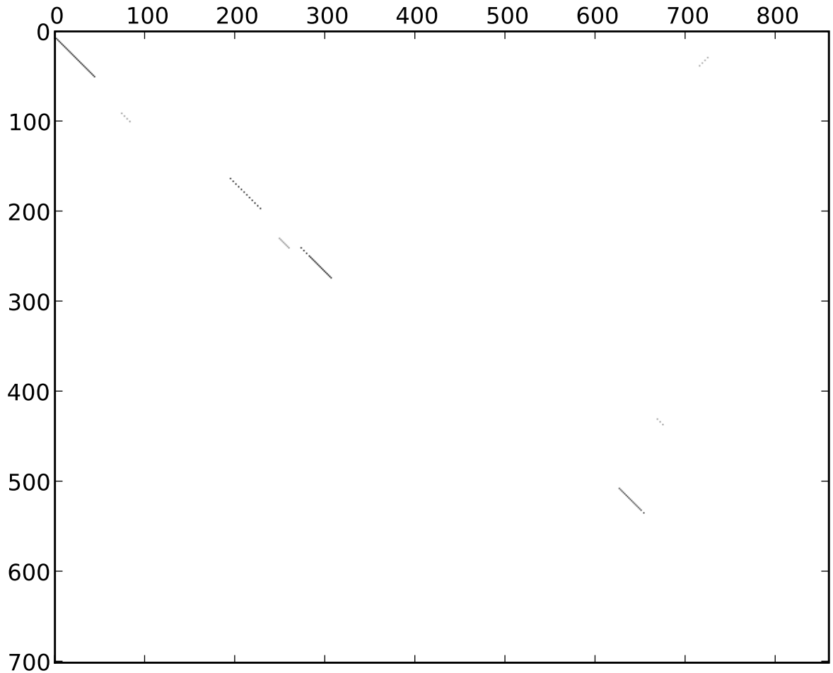
st2_dmel_dvir_blastplot_9_rev_normed
