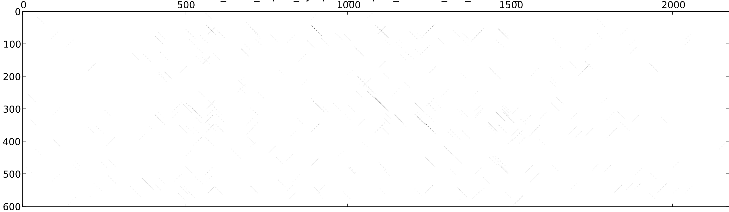
st37_dmel_sepsis_cynipsea_dotplot_20-0.60_rev_normed_extend
