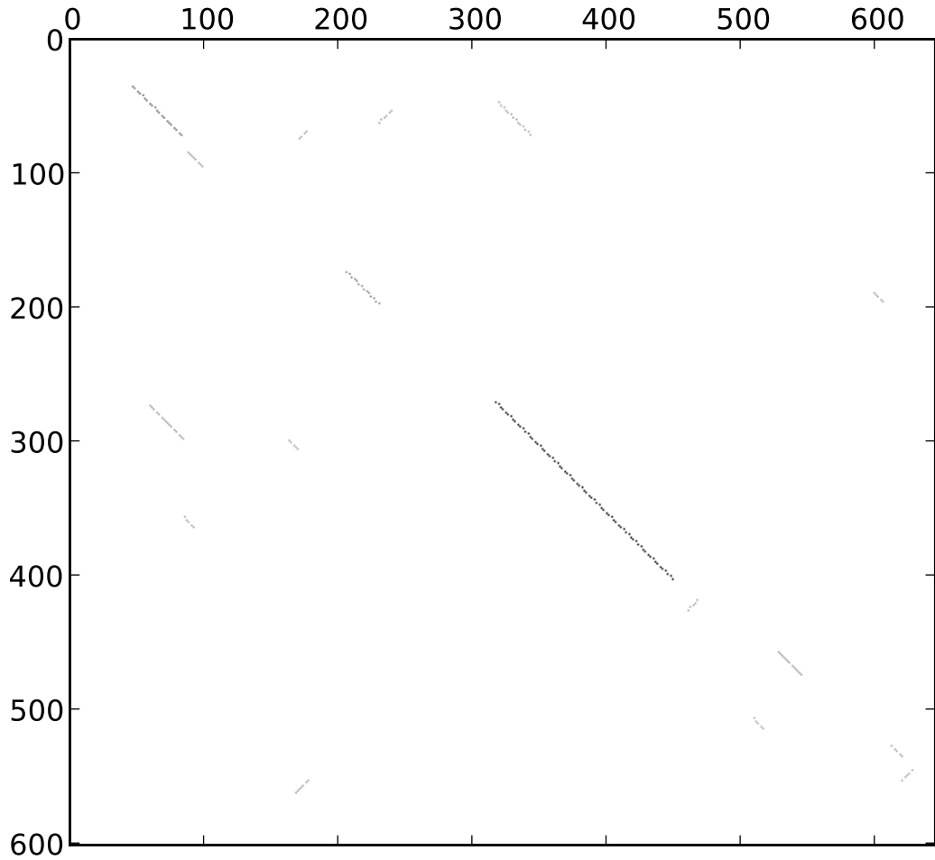
st37_dmel_dpse_blastplot_9_rev_normed
