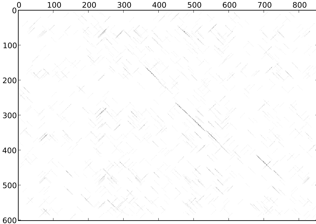
st37_dmel_dvir_dotplot_14-0.60_rev_normed_extend
