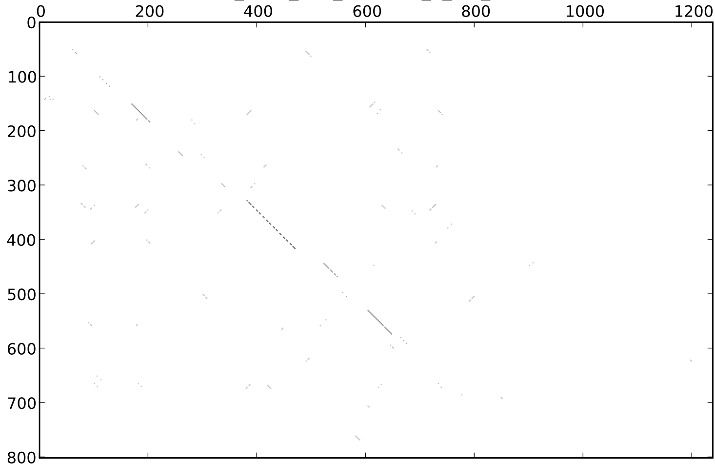
st46_dmel_dvir_blastplot_7_rev_normed
