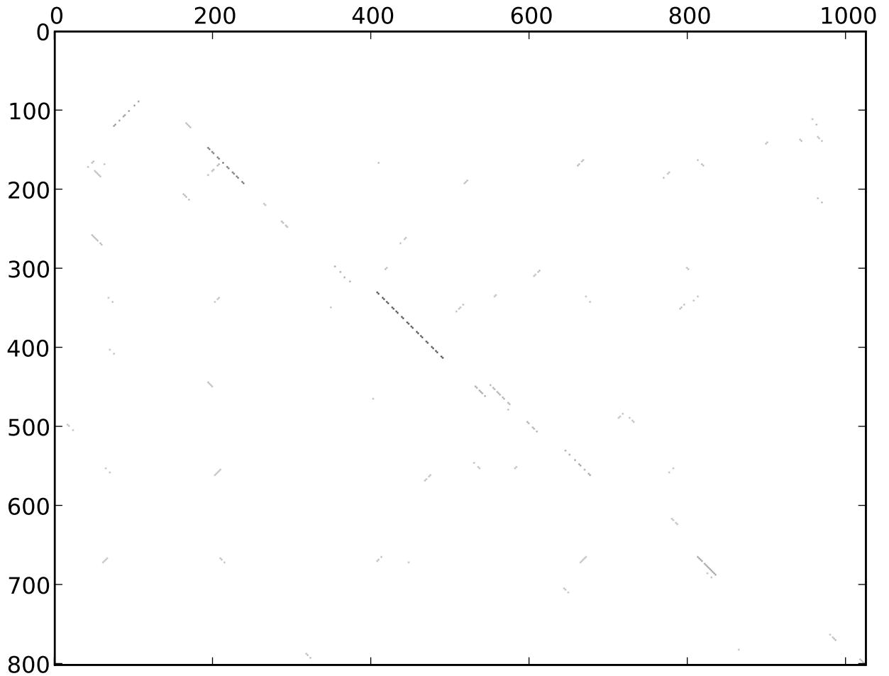
st46_dmel_dpse_blastplot_7_rev_normed
