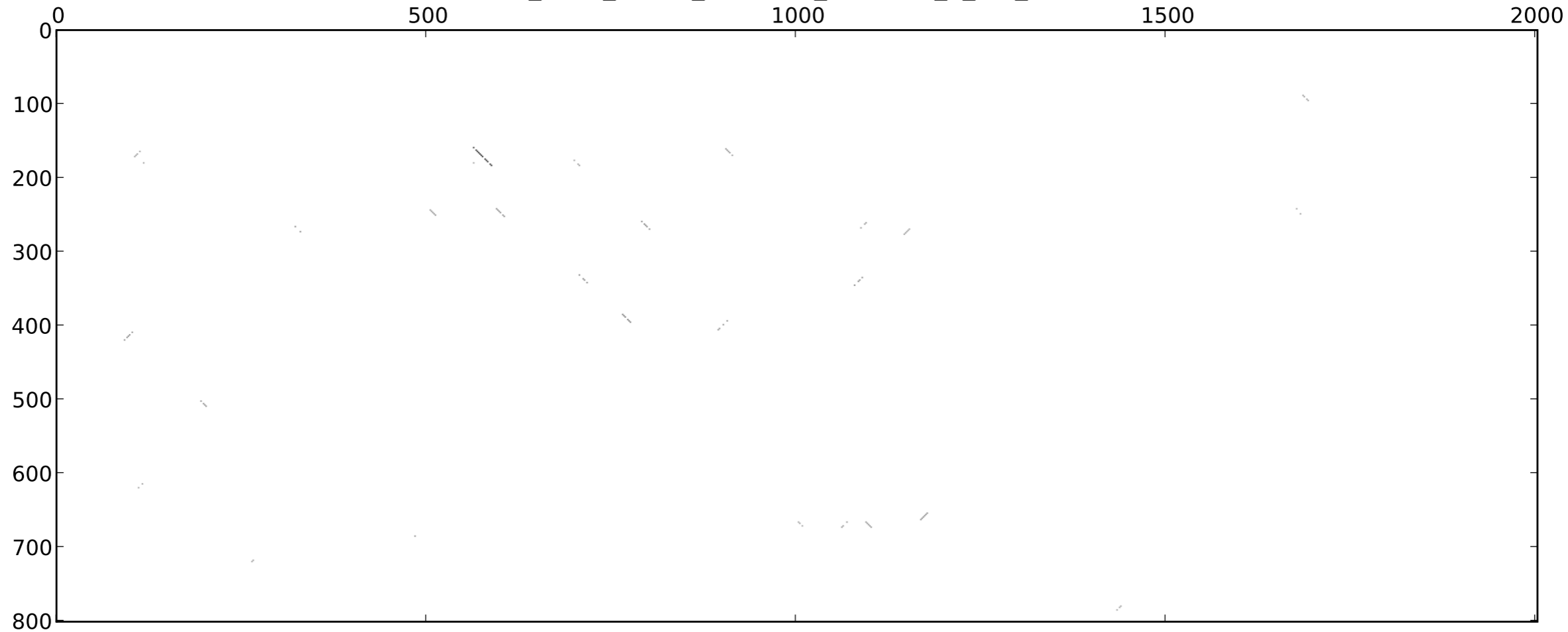
st46_dmel_sepsis_cynipsea_blastplot_7_rev_normed
