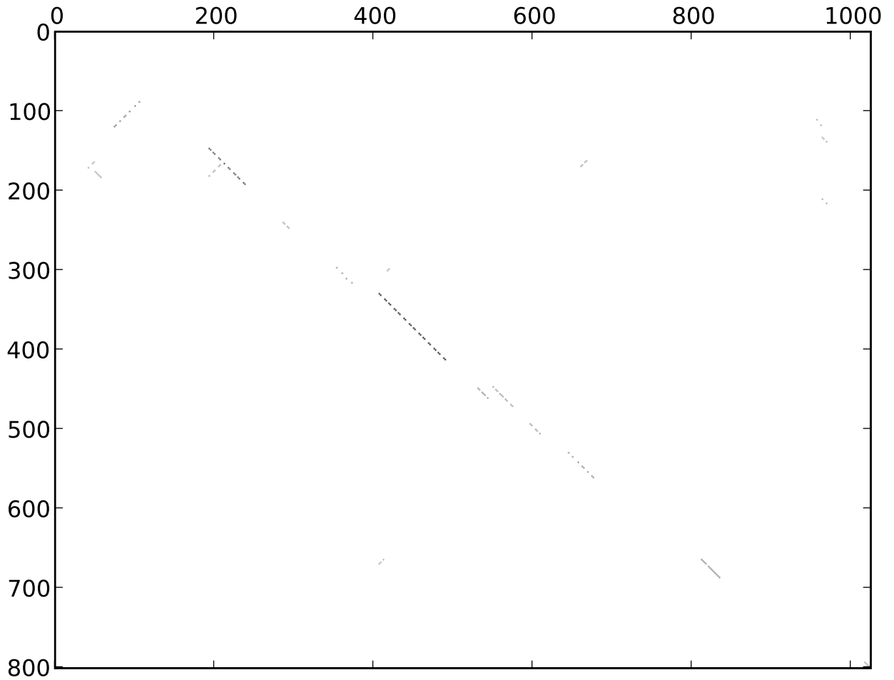
st46_dmel_dpse_blastplot_9_rev_normed
