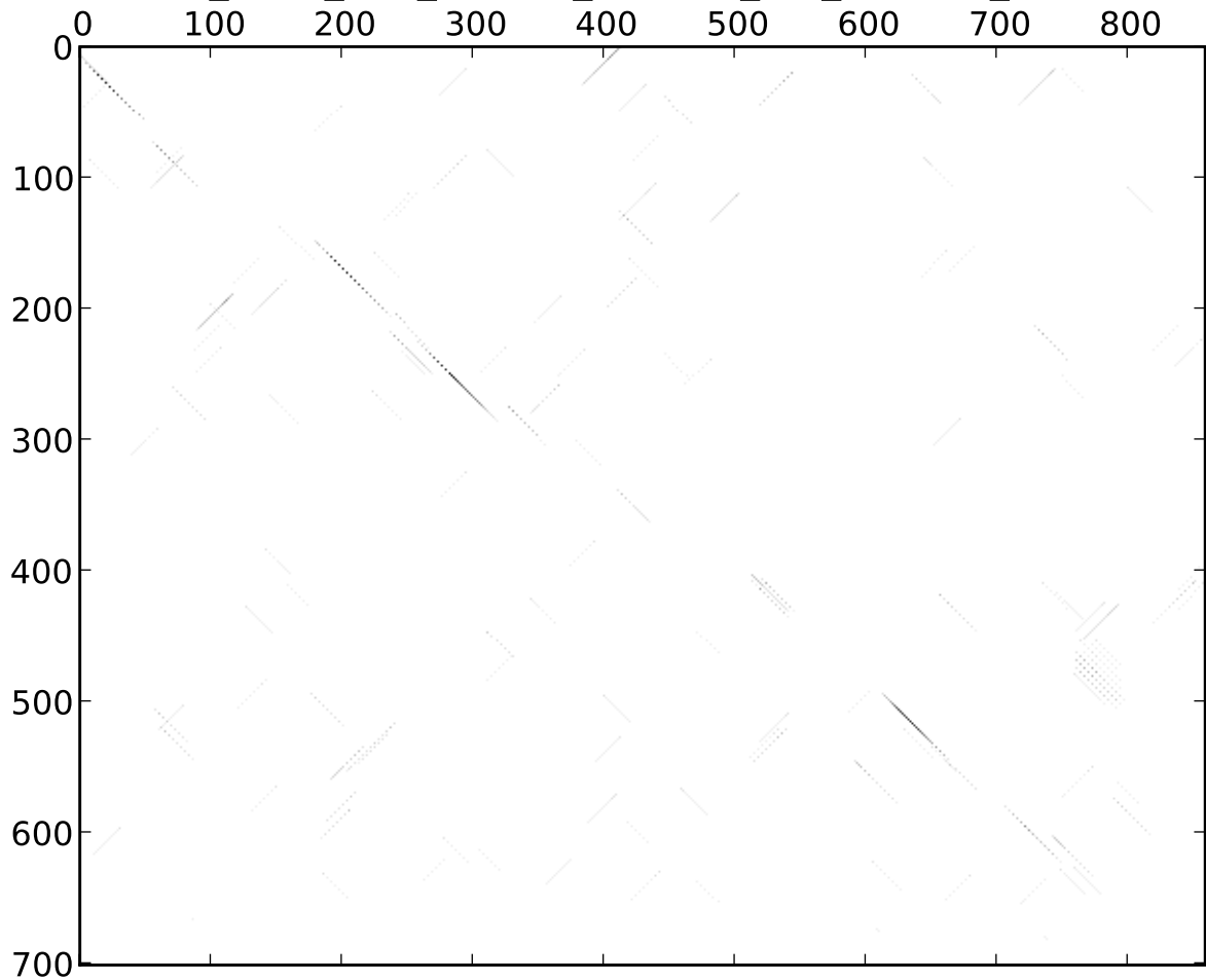
st2_dmel_dvir_dotplot_20-0.60_rev_normed_extend
