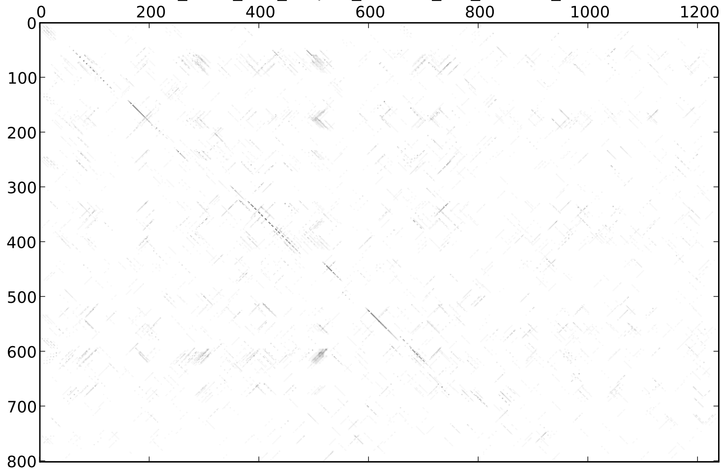
st46_dmel_dvir_dotplot_14-0.60_rev_normed_extend
