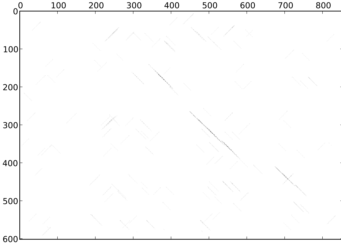
st37_dmel_dvir_dotplot_20-0.60_rev_normed_extend
