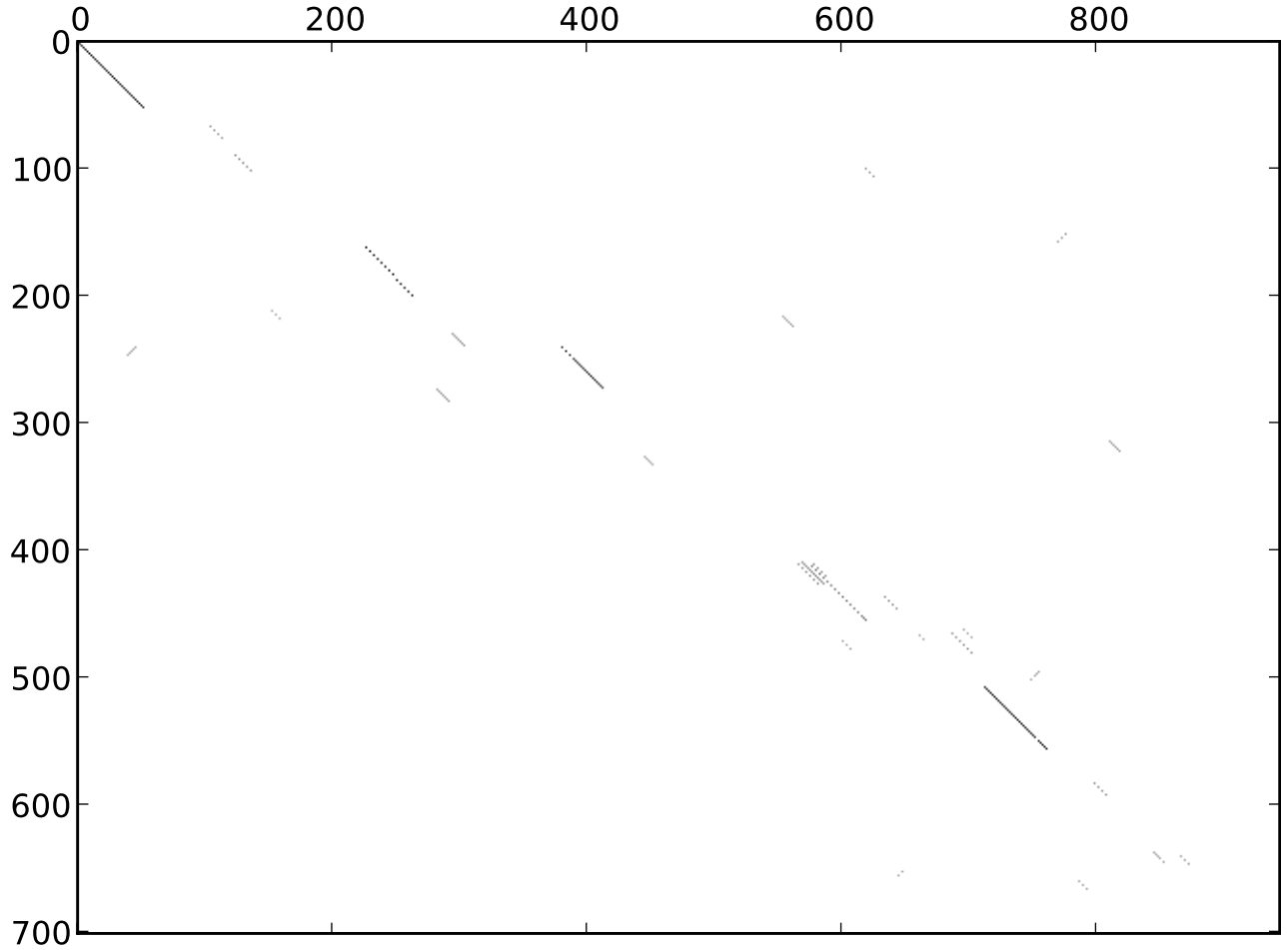
st2_dmel_dpse_blastplot_7_rev_normed
