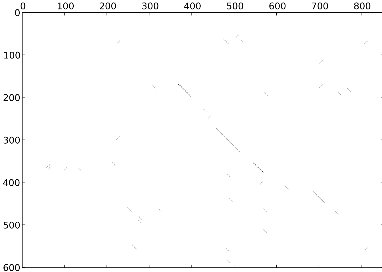
st37_dmel_dvir_blastplot_7_rev_normed
