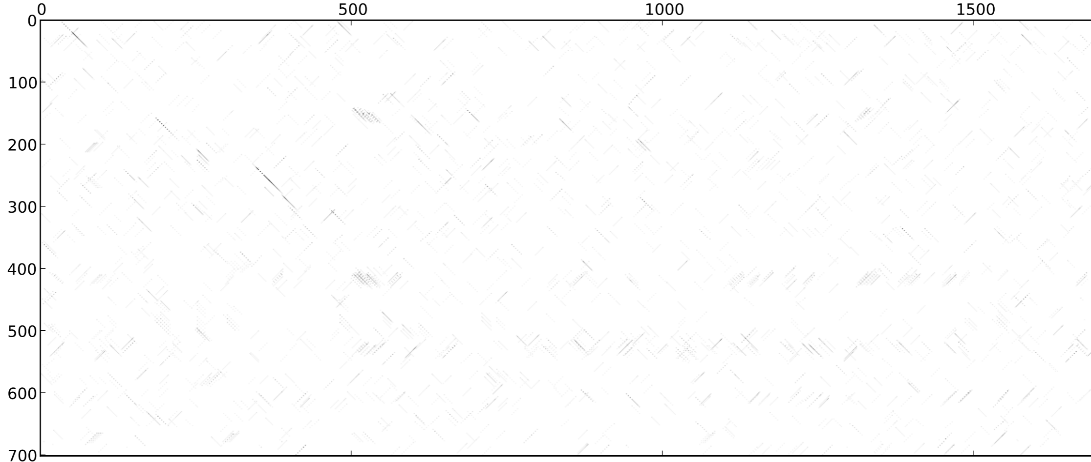
st2_dmel_themira_putris_dotplot_14-0.60_rev_normed_extend
