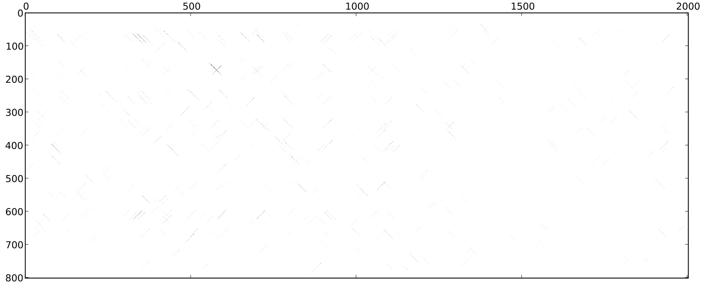
st46_dmel_sepsis_cynipsea_dotplot_20-0.60_rev_normed_extend
