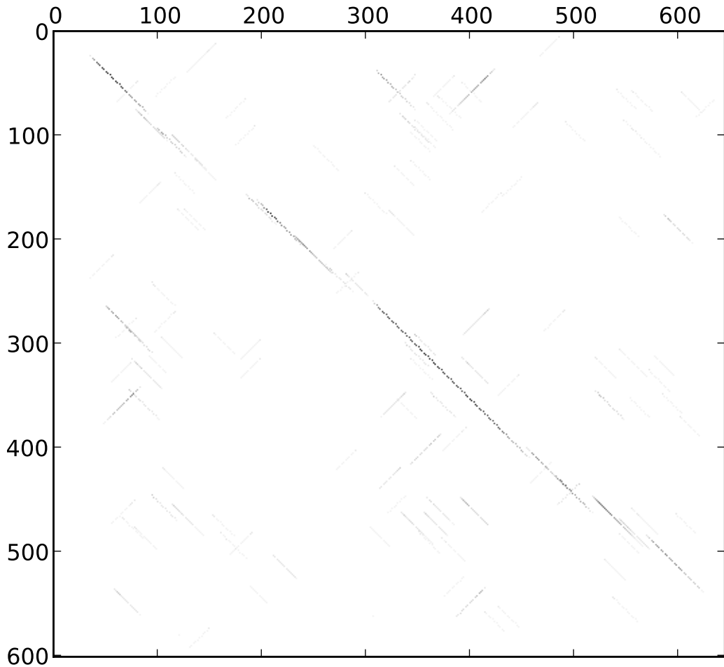
st37_dmel_dpse_dotplot_20-0.60_rev_normed_extend
