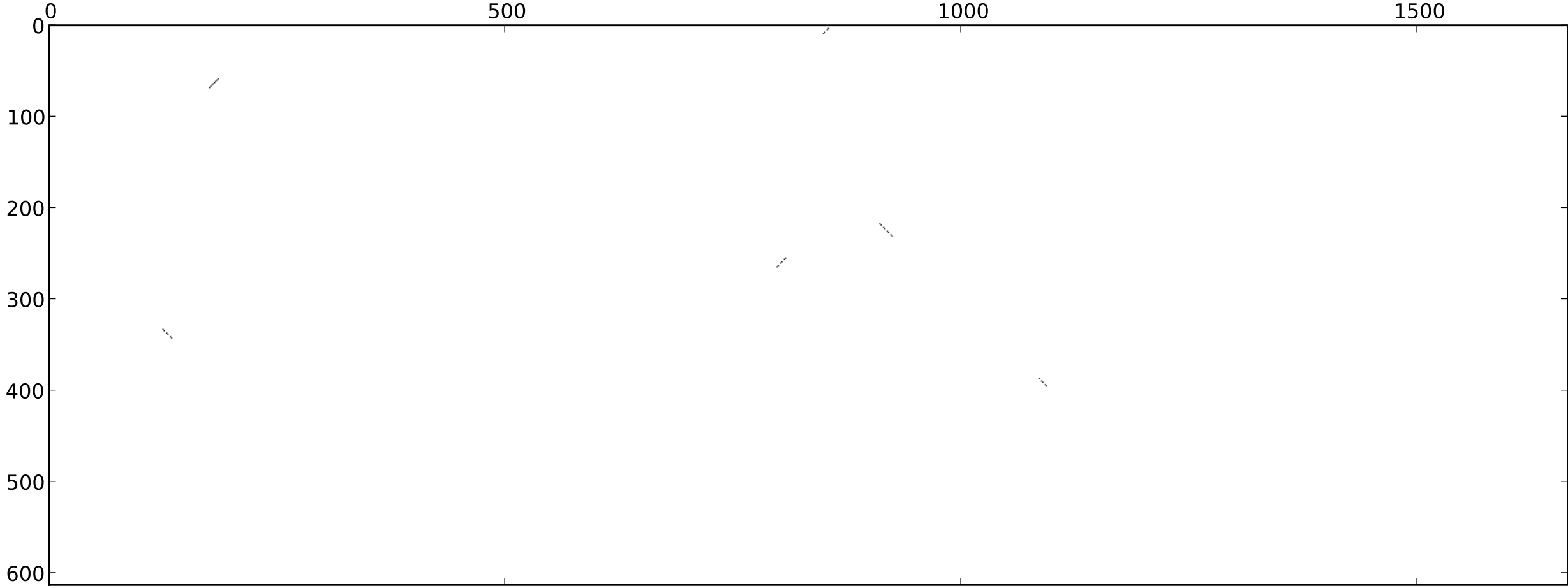
MHE_dmel_themira_putris_blastplot_9_rev_normed
