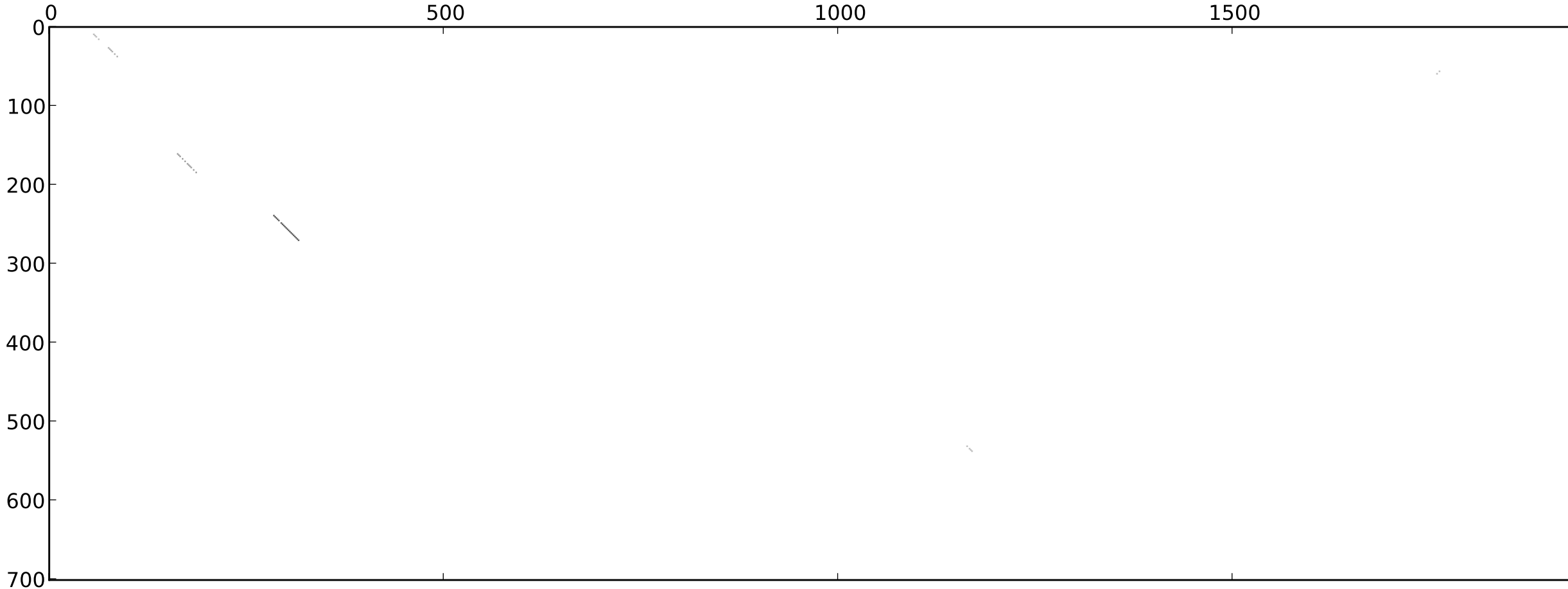
st2_dmel_sepsis_cynipsea_blastplot_9_rev_normed
