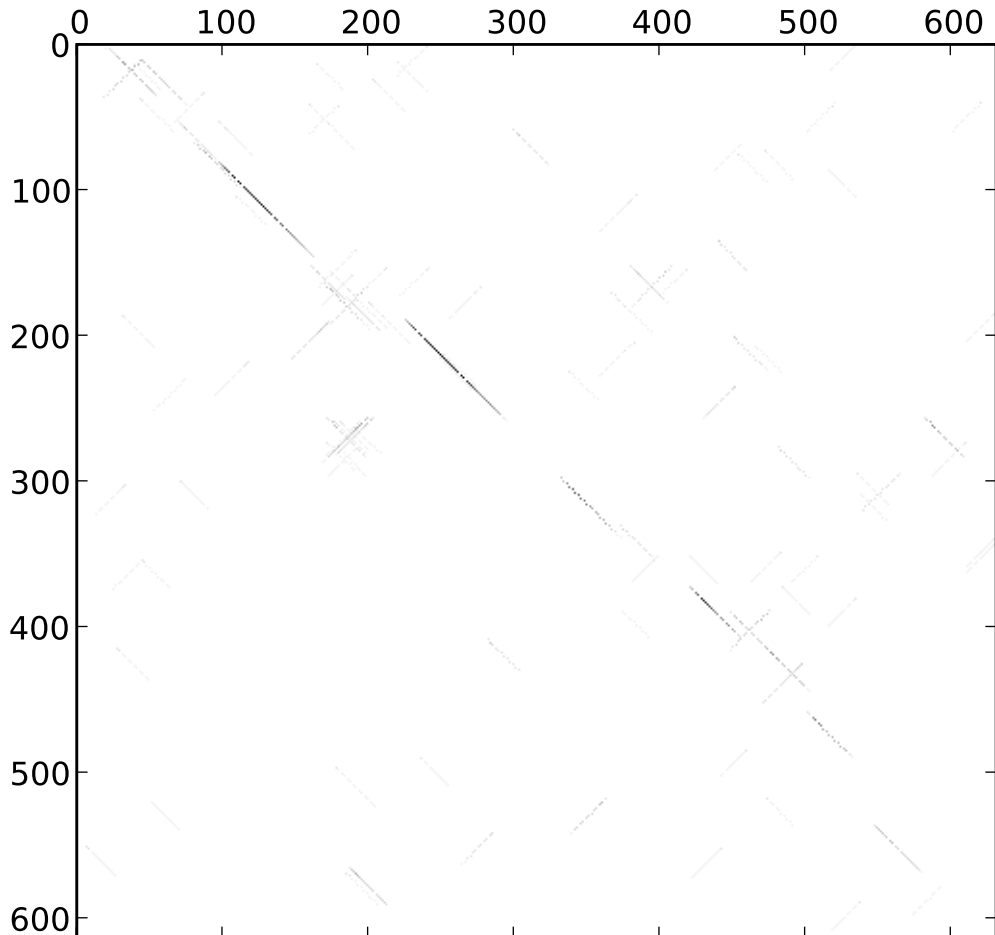
MHE_dmel_dpse_dotplot_20-0.60_rev_normed_extend
