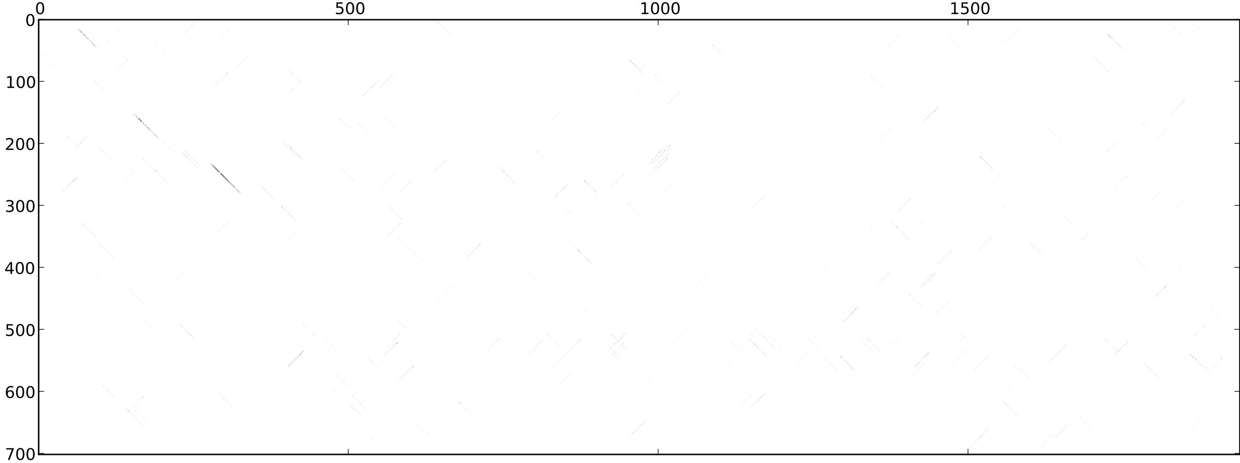
st2_dmel_sepsis_cynipsea_dotplot_20-0.60_rev_normed_extend
