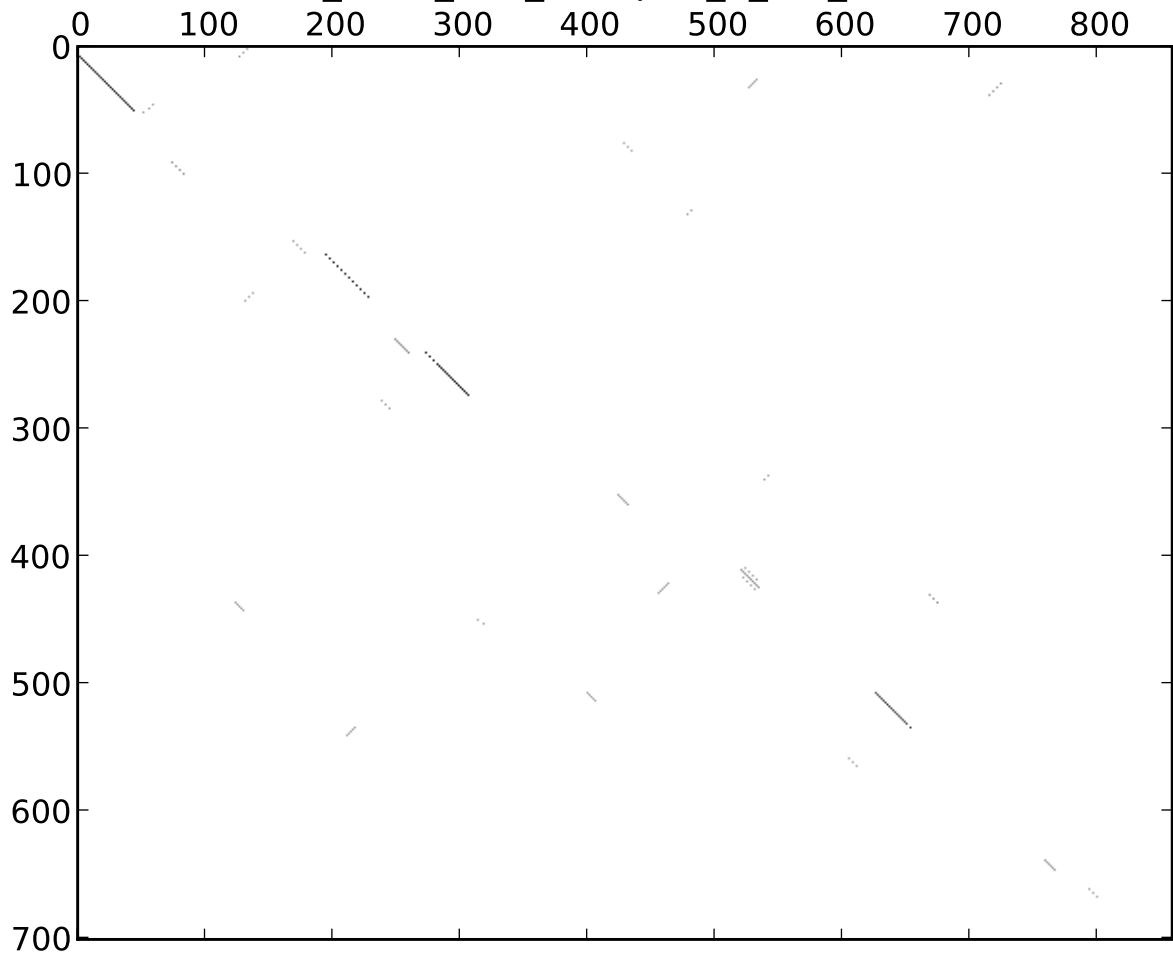
st2_dmel_dvir_blastplot_7_rev_normed
