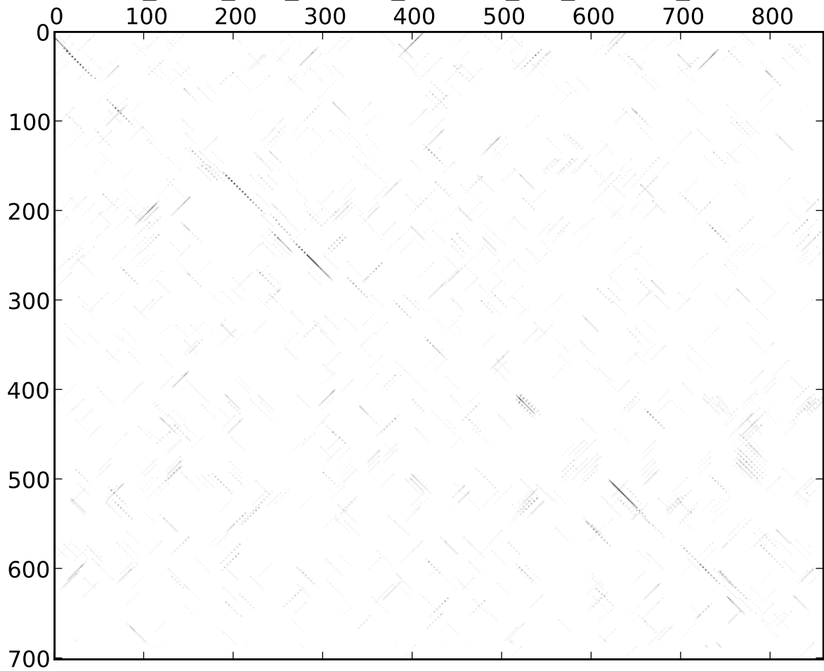
st2_dmel_dvir_dotplot_14-0.60_rev_normed_extend
