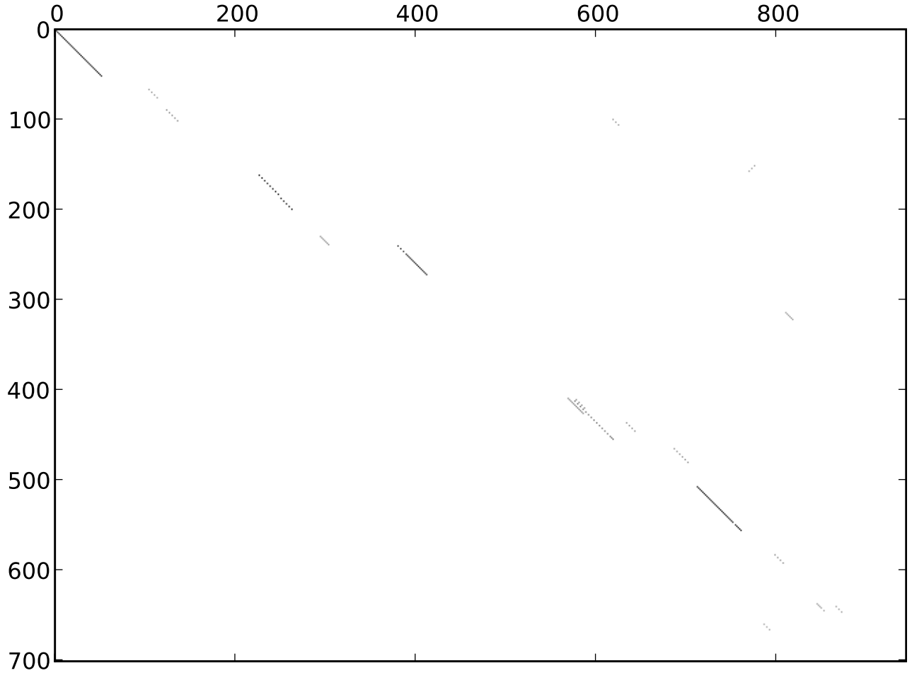
st2_dmel_dpse_blastplot_9_rev_normed
