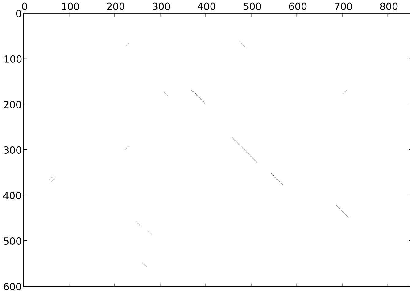
st37_dmel_dvir_blastplot_9_rev_normed
