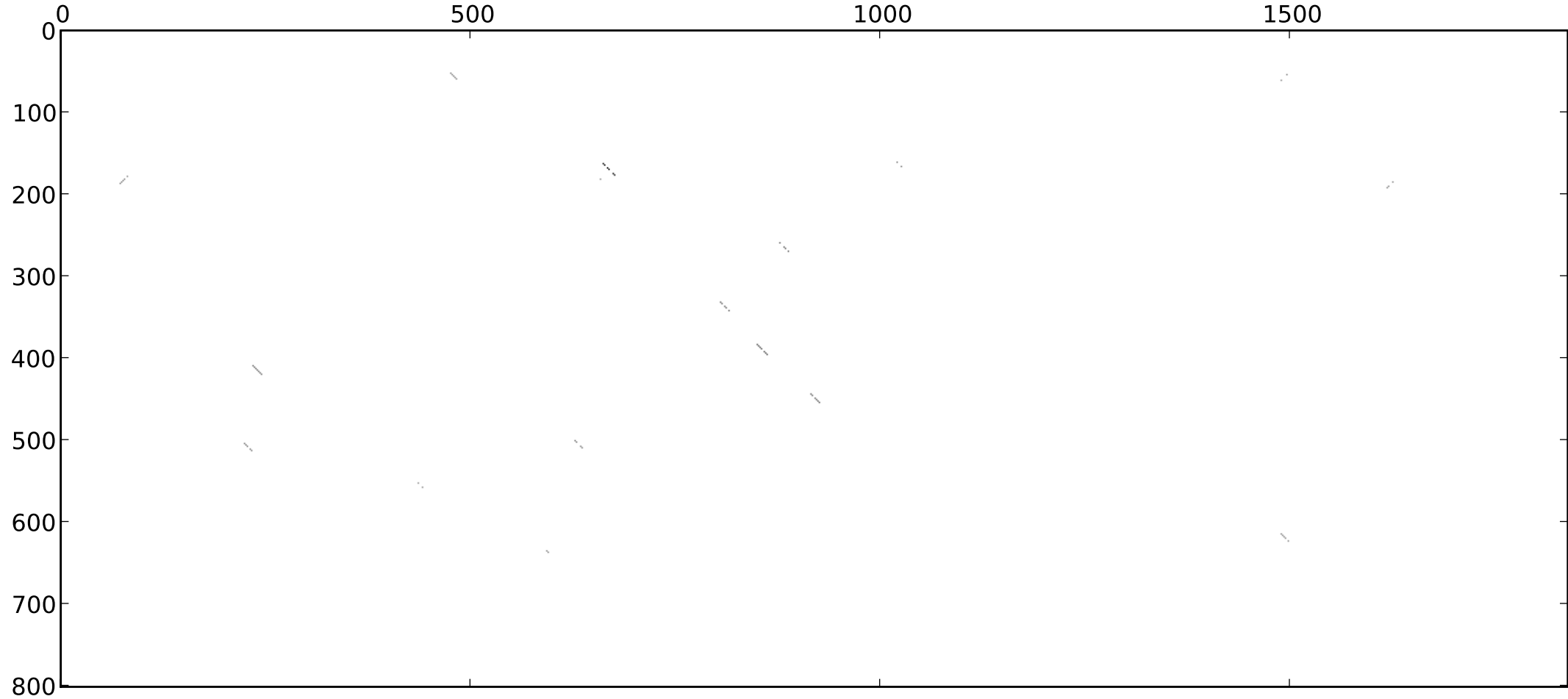
st46_dmel_themira_putris_blastplot_9_rev_normed
