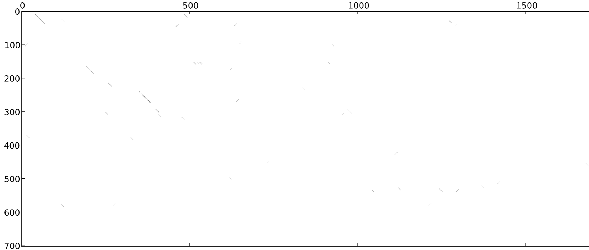
st2_dmel_themira_putris_blastplot_7_rev_normed
