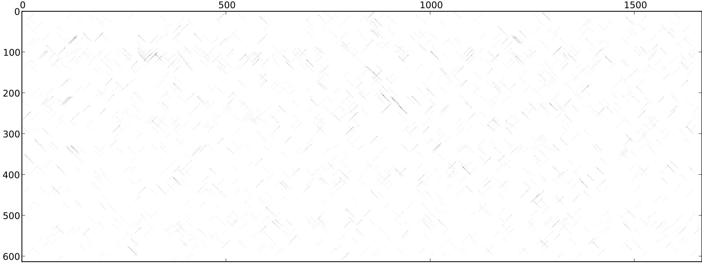
MHE_dmel_themira_putris_dotplot_14-0.60_rev_normed_extend
