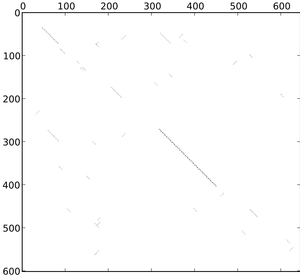
st37_dmel_dpse_blastplot_7_rev_normed
