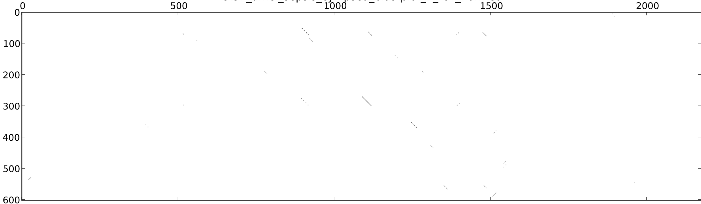
st37_dmel_sepsis_cynipsea_blastplot_7_rev_normed
