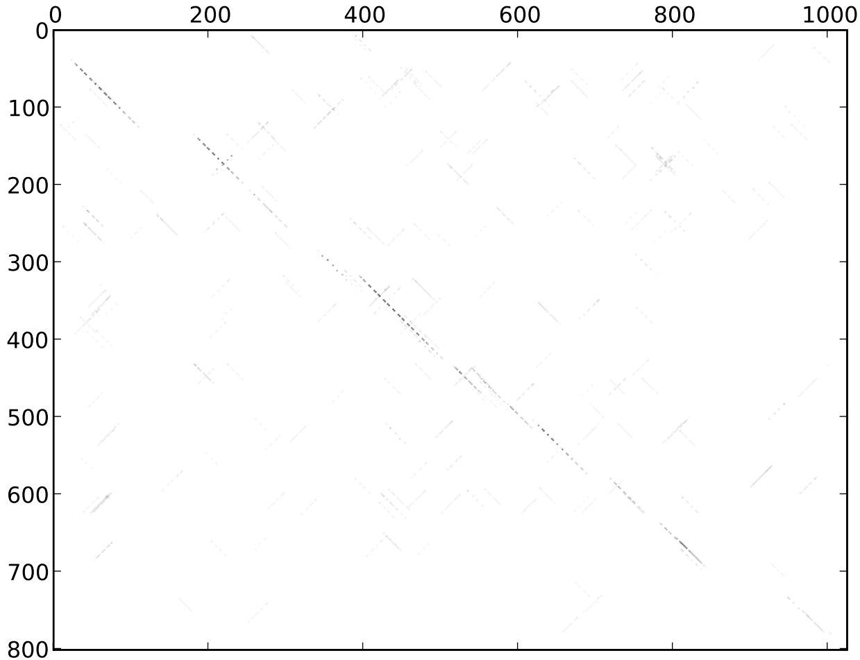
st46_dmel_dpse_dotplot_20-0.60_rev_normed_extend
