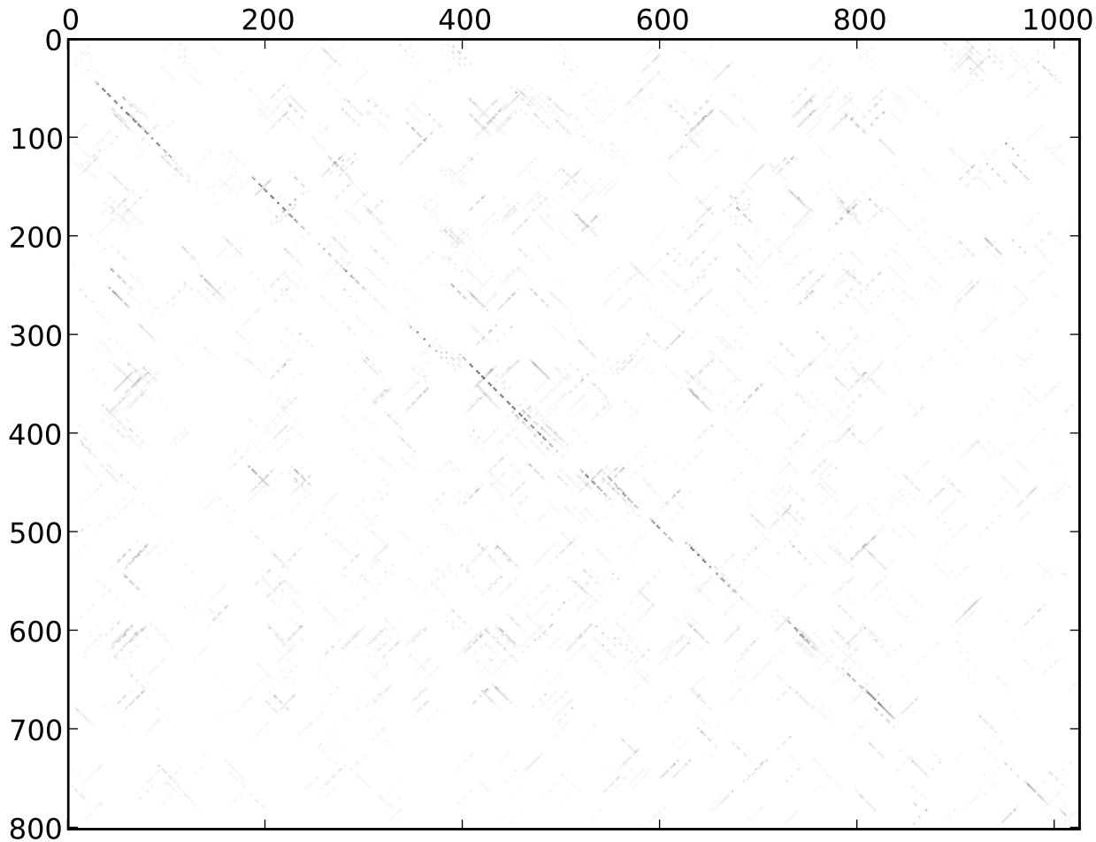
st46_dmel_dpse_dotplot_14-0.60_rev_normed_extend
