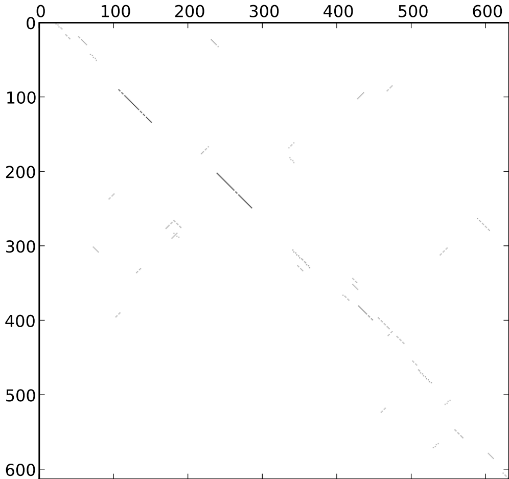
MHE_dmel_dpse_blastplot_7_rev_normed
