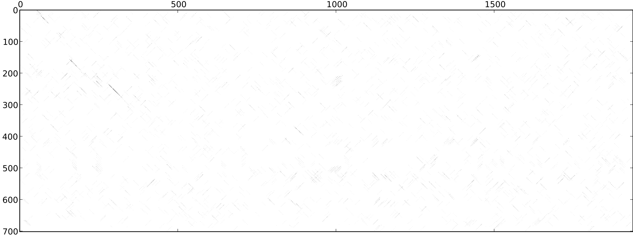
st2_dmel_sepsis_cynipsea_dotplot_14-0.60_rev_normed_extend
