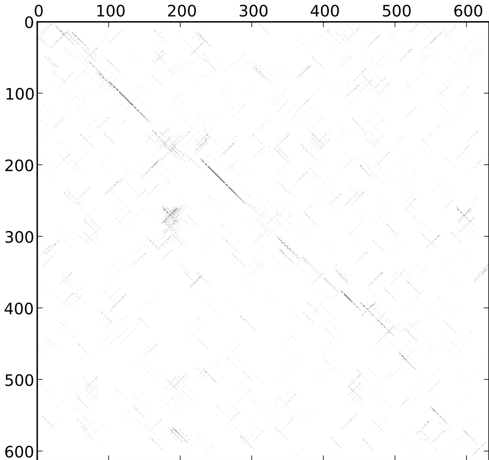
MHE_dmel_dpse_dotplot_14-0.60_rev_normed_extend
