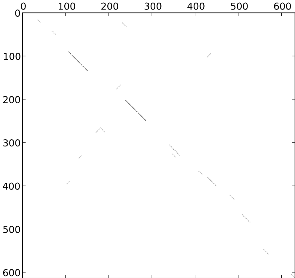
MHE_dmel_dpse_blastplot_9_rev_normed
