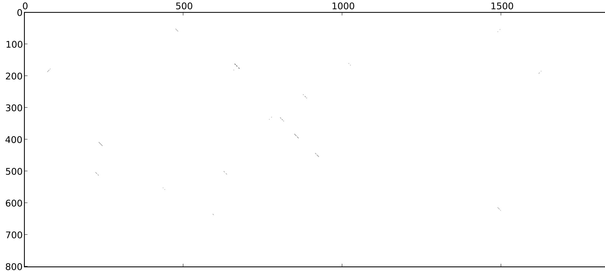
st46_dmel_themira_putris_blastplot_7_rev_normed
