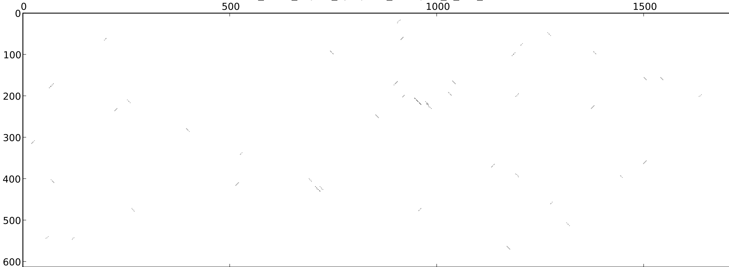
MHE_dmel_sepsis_cynipsea_blastplot_7_rev_normed
