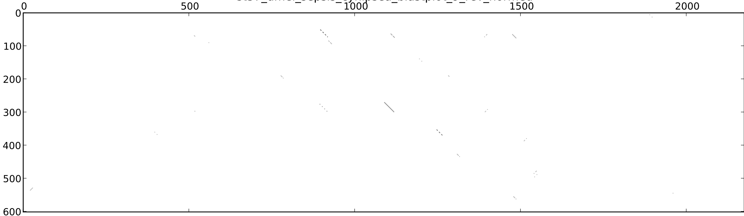
st37_dmel_sepsis_cynipsea_blastplot_9_rev_normed
