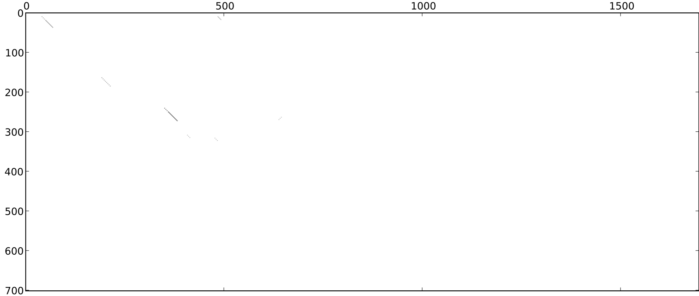
st2_dmel_themira_putris_blastplot_9_rev_normed
