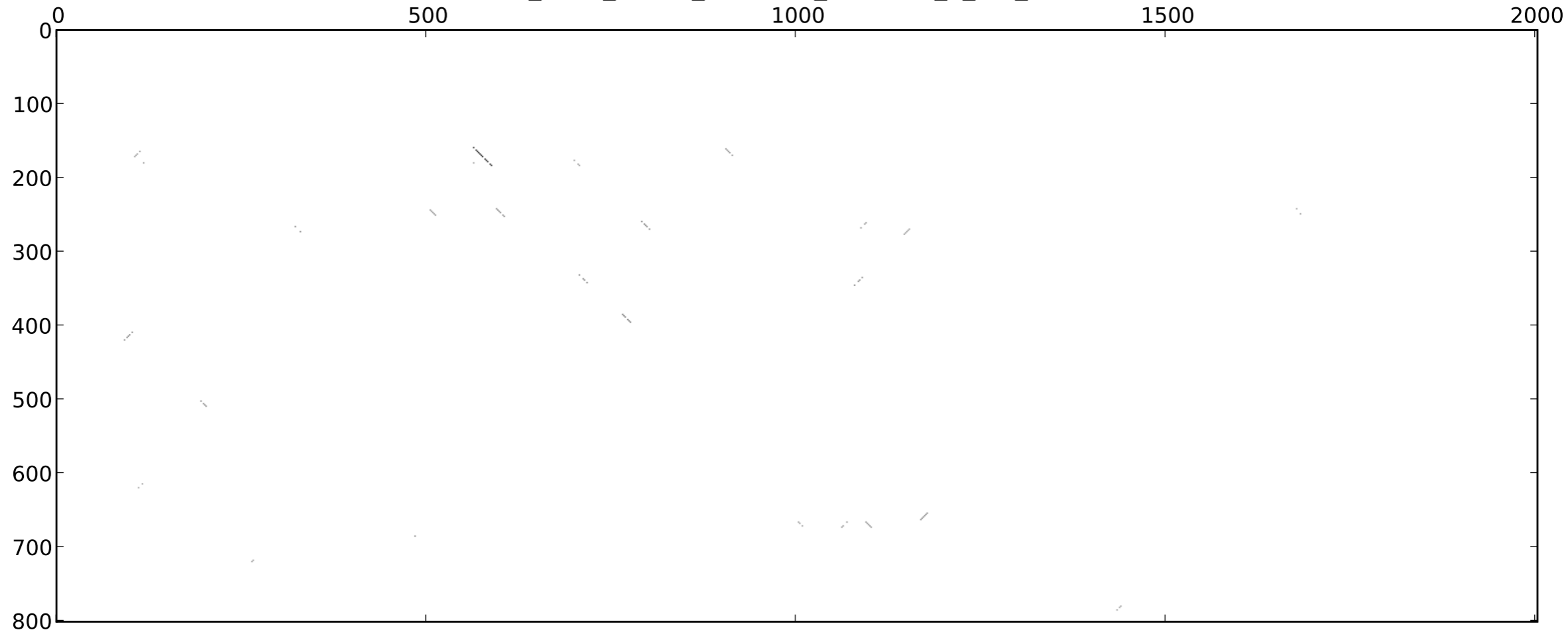
st46_dmel_sepsis_cynipsea_blastplot_9_rev_normed
