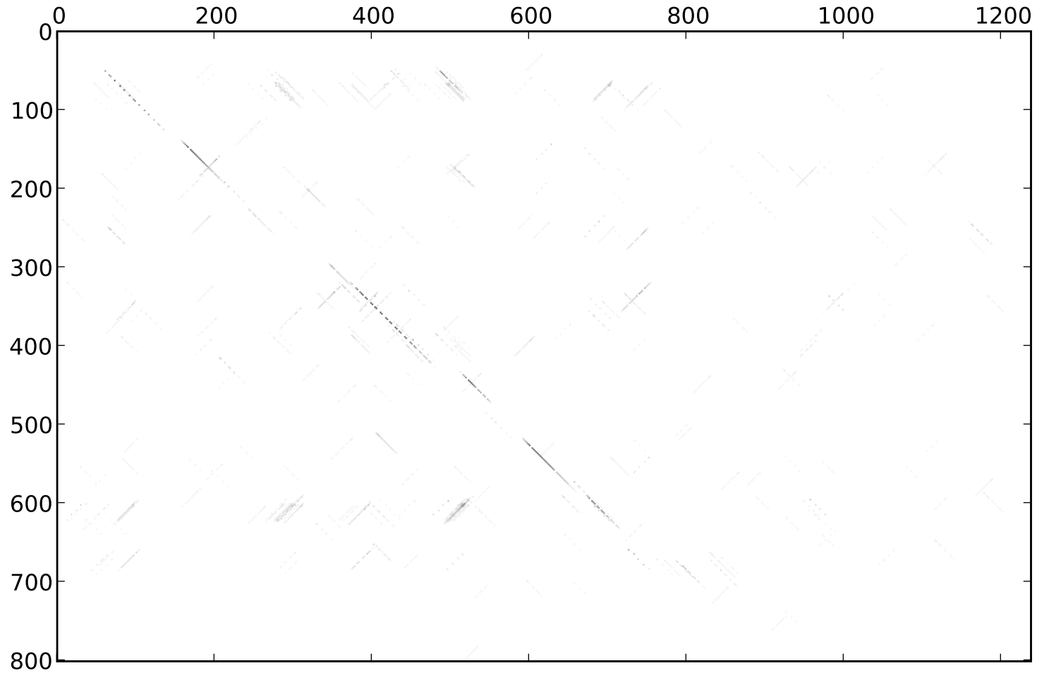
st46_dmel_dvir_dotplot_20-0.60_rev_normed_extend
