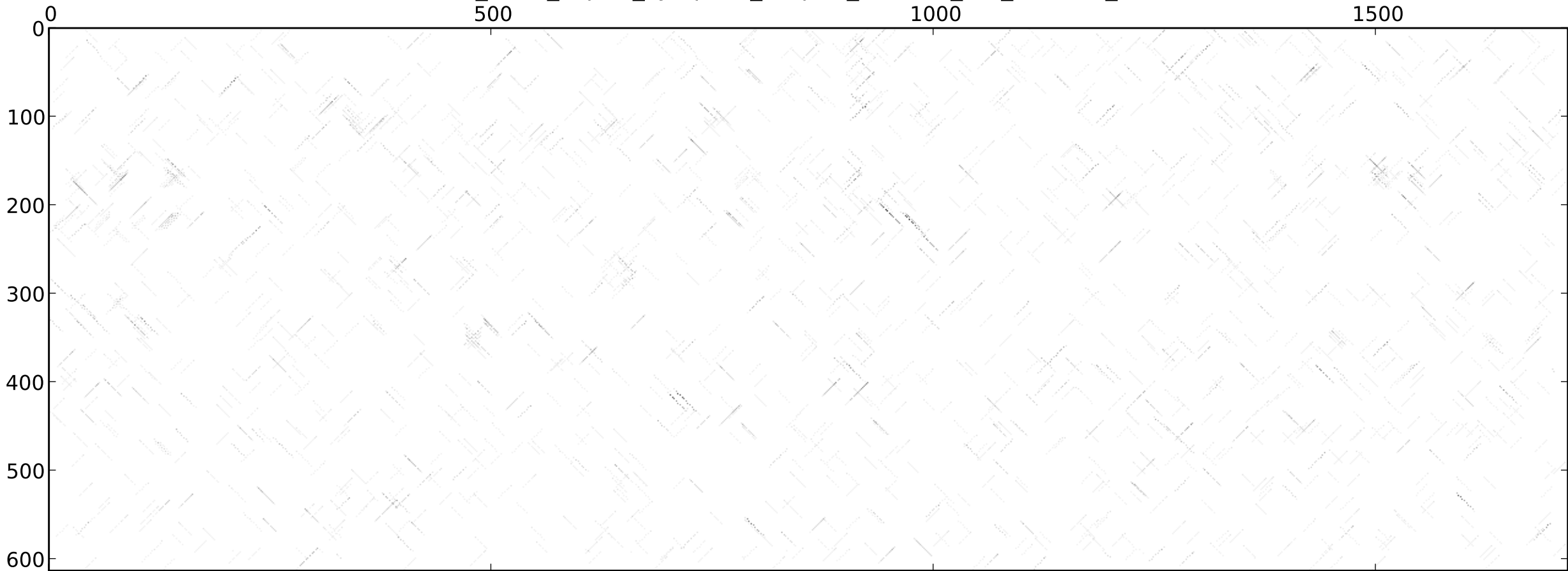
MHE_dmel_sepsis_cynipsea_dotplot_14-0.60_rev_normed_extend
