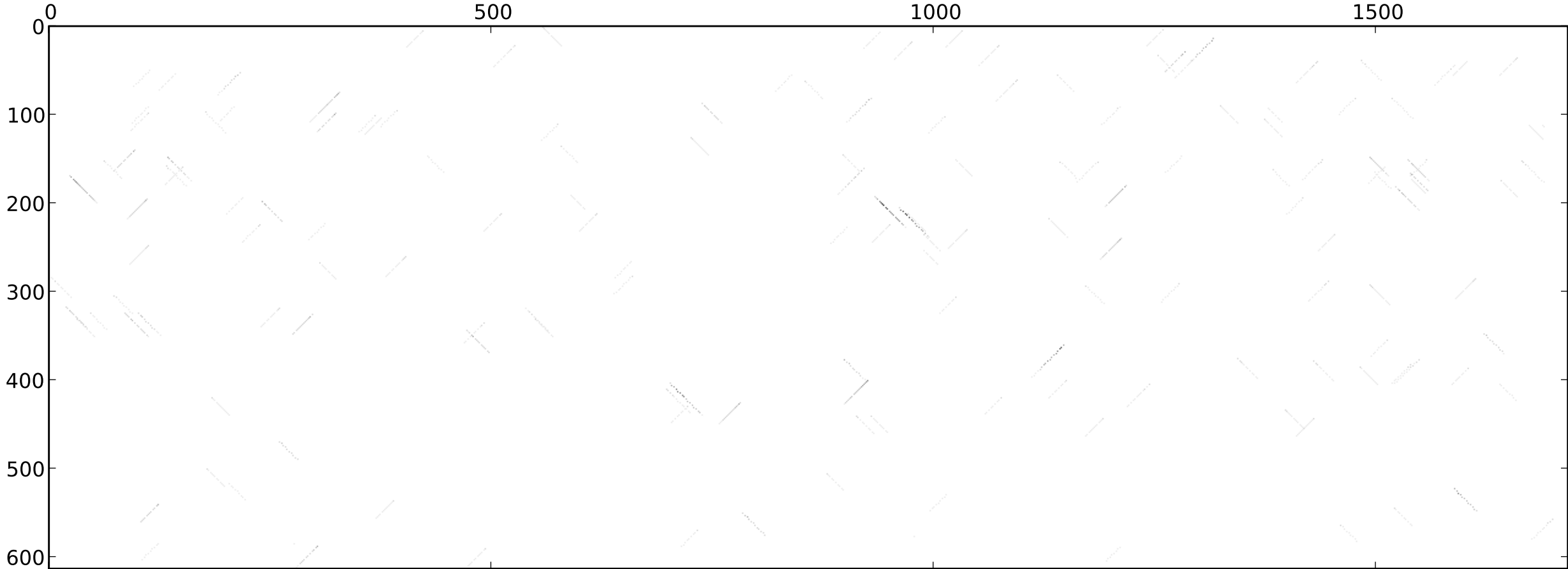
MHE_dmel_sepsis_cynipsea_dotplot_20-0.60_rev_normed_extend
