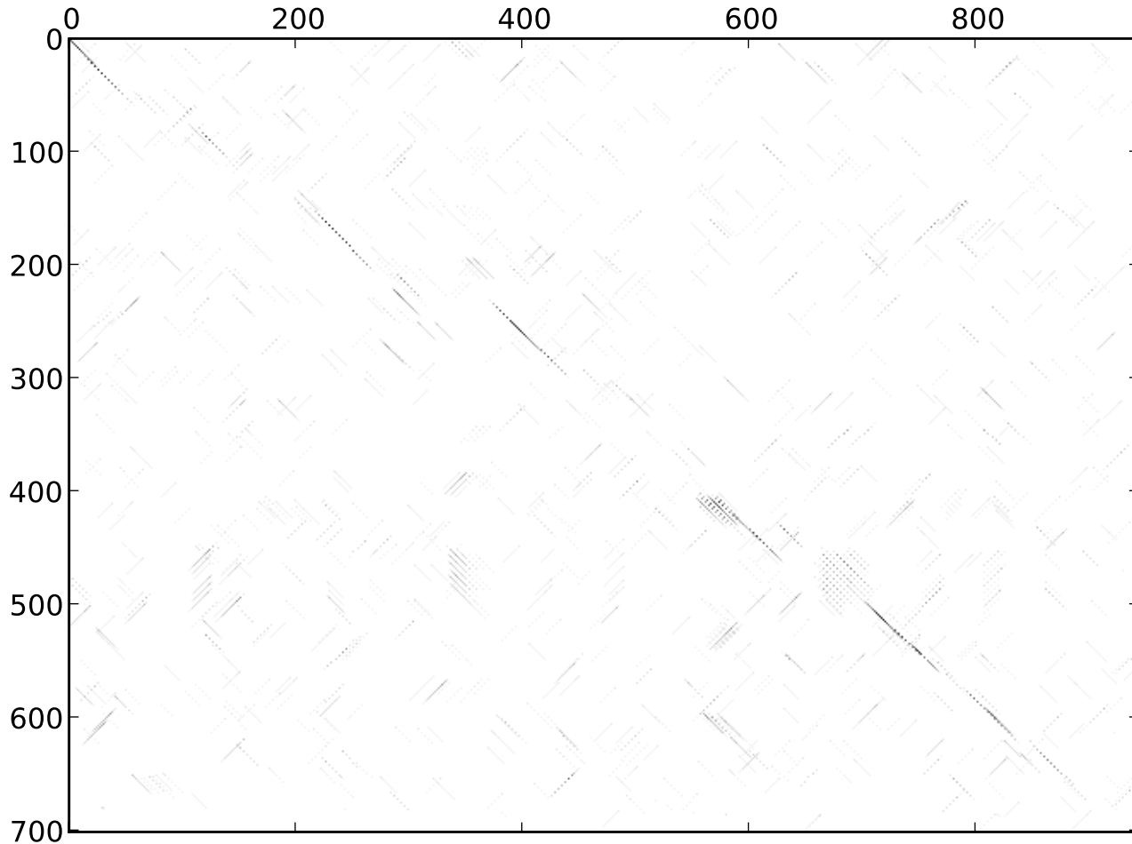
st2_dmel_dpse_dotplot_14-0.60_rev_normed_extend
