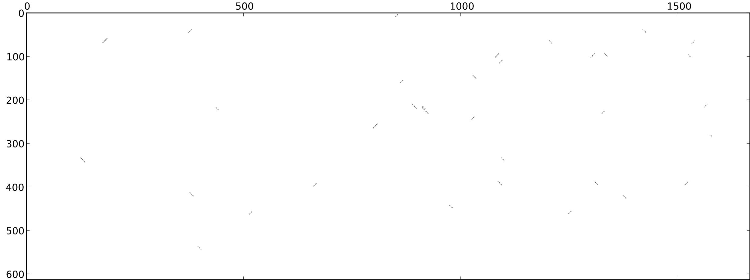
MHE_dmel_themira_putris_blastplot_7_rev_normed
