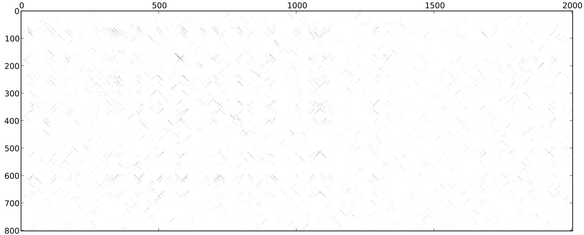
st46_dmel_sepsis_cynipsea_dotplot_14-0.60_rev_normed_extend
