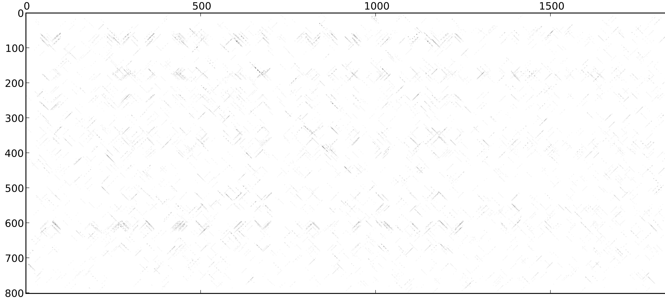
st46_dmel_themira_putris_dotplot_14-0.60_rev_normed_extend
