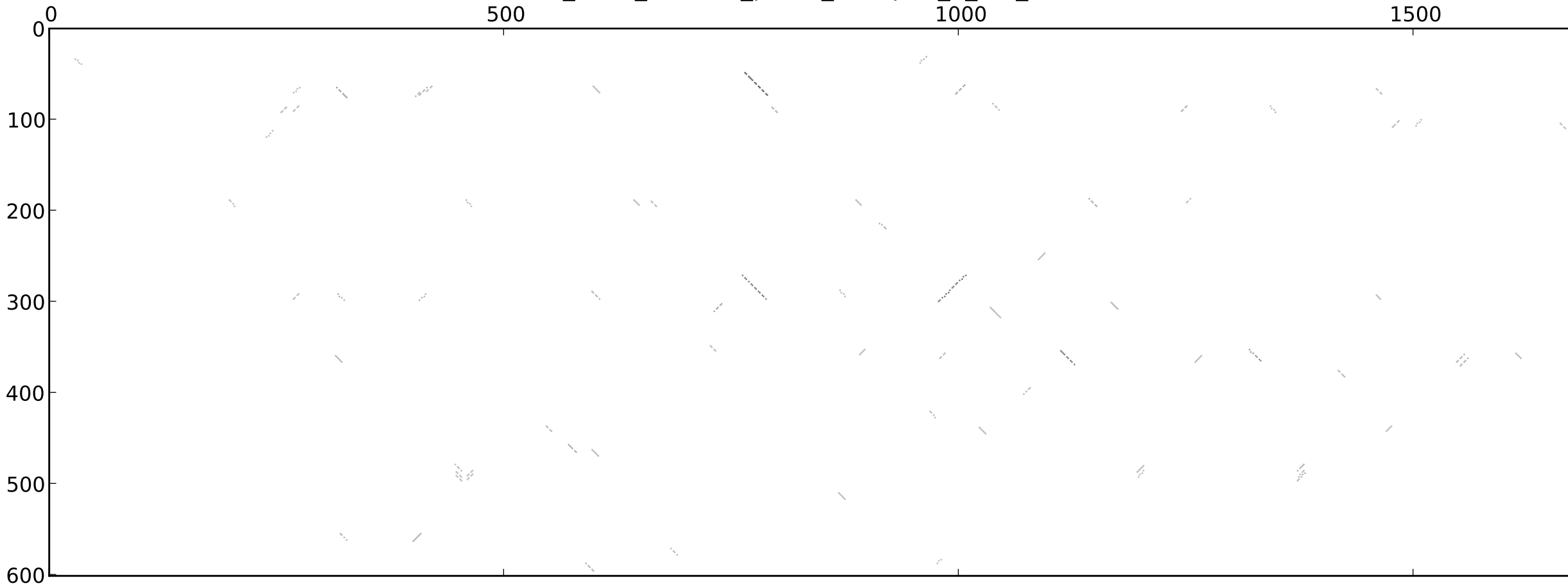
st37_dmel_themira_putris_blastplot_7_rev_normed
