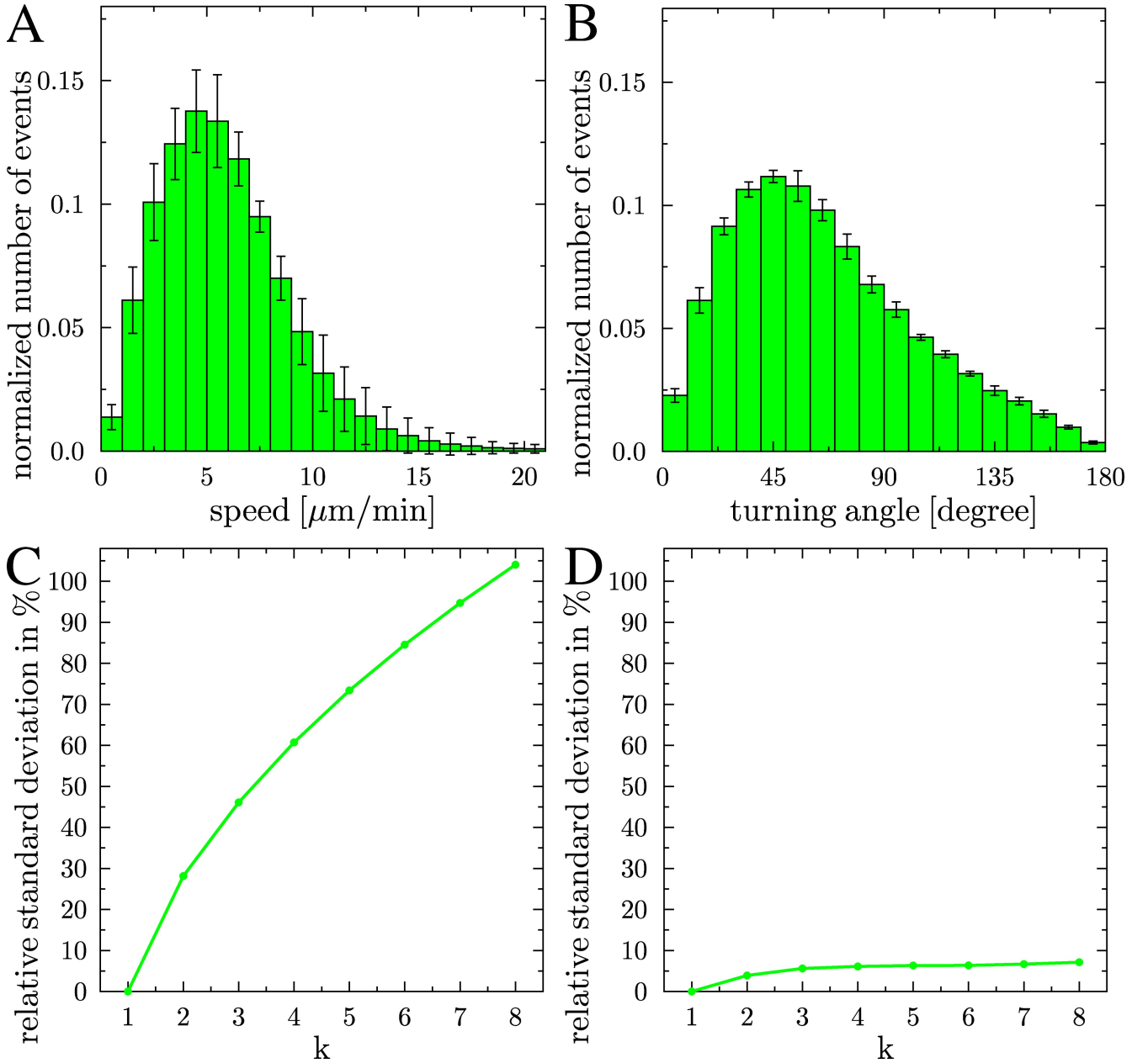
Figure S2. Normalized speed and turning angle distributions as obtained from averaging over different time resolutions. (A) The speed distribution changes with a mean relative SD of \sim 70\% . (B) The turning angle distribution is robust with a mean relative SD of \sim 6\% . (C) The mean relative standard deviation for the speed distribution is an increasing function of the total number included time resolutions k . (D) The mean relative standard deviation for the turning angle distribution as a function of k shows its robustness with respect to the time resolution of the cell track evaluation.
