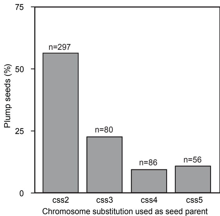
Supplemental figure S2. Substitution of Ler chromosome two in a Col background (C ss2 ) dramatically increases the frequency of live seed in the progeny of crosses to tetraploid Col (Y axis). No other chromosome provided a dramatic increase over the control 2x Col X 4x Col crosses (Figure 1).
