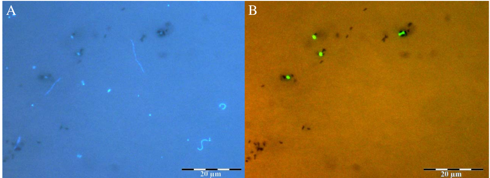
Fig. S1 Images of whole cell hybridization combined with microautoradiography of the Black Sea (125m depth) incubated with [ 14 C]bicarbonate. A DAPI-stained bacteria; B bacteria hybridized with oligonucleotide probe EPS914 specific for Epsilonproteobacteria . Accumulation of dark silver grains around the cells indicate dark CO 2 fixation activity. Images show the same microscopic view.
