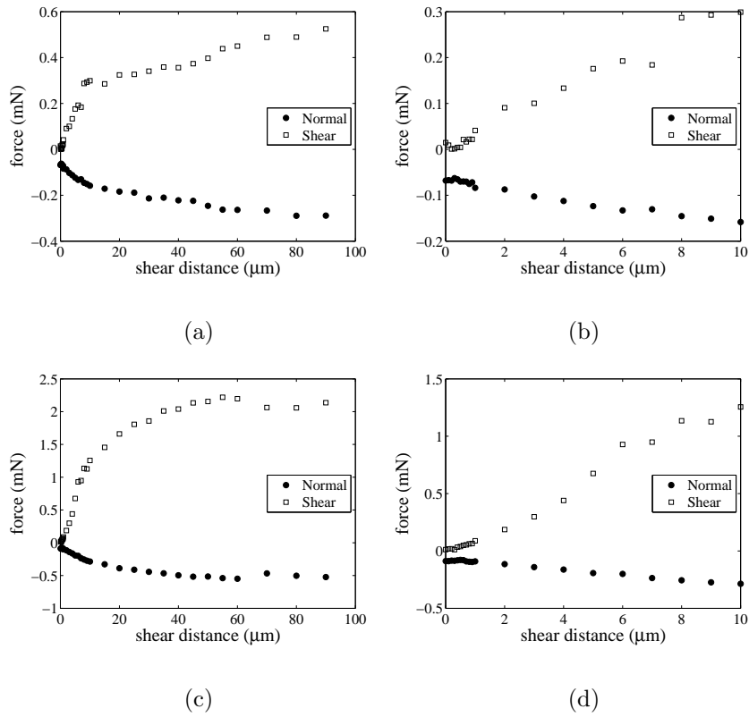
Figure 1. Data points represent the shear force measured at the highest pull-off value for LDP experiments performed with different shear distances. Preloads were (a,b) 0.5 mN and (c,d) 2.0 mN. Plots (b) and (d) are close-ups of plots (a) and (c), respectively.
