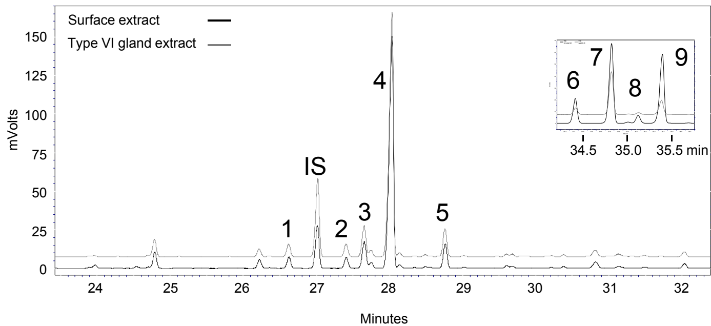
Supplemental Figure S1. Terpenoid accumulation in type VI trichomes of S. habrochaites LA1777. Overlay of GC chromatograms (TIC) of extracts from leaf surface (black) and type VI glands (grey). Inset: Separate chromatograms of TMCS-derivatized cII-SCAs. IS, internal standard (tetradecane); 1, \beta -elemene; 2, \alpha -cis-bergamotene; 3, \alpha -cis-santalene; 4, \gamma -elemene; 5, unknown; 6, \alpha -cis-bergamotenoic acid; 7, \alpha -cis-santalenoic acid; 8, \alpha -trans-bergamotenoic acid; 9, \beta -cis-bergamotenoic acid.
