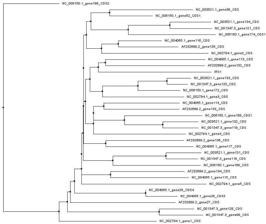
ClustalW
