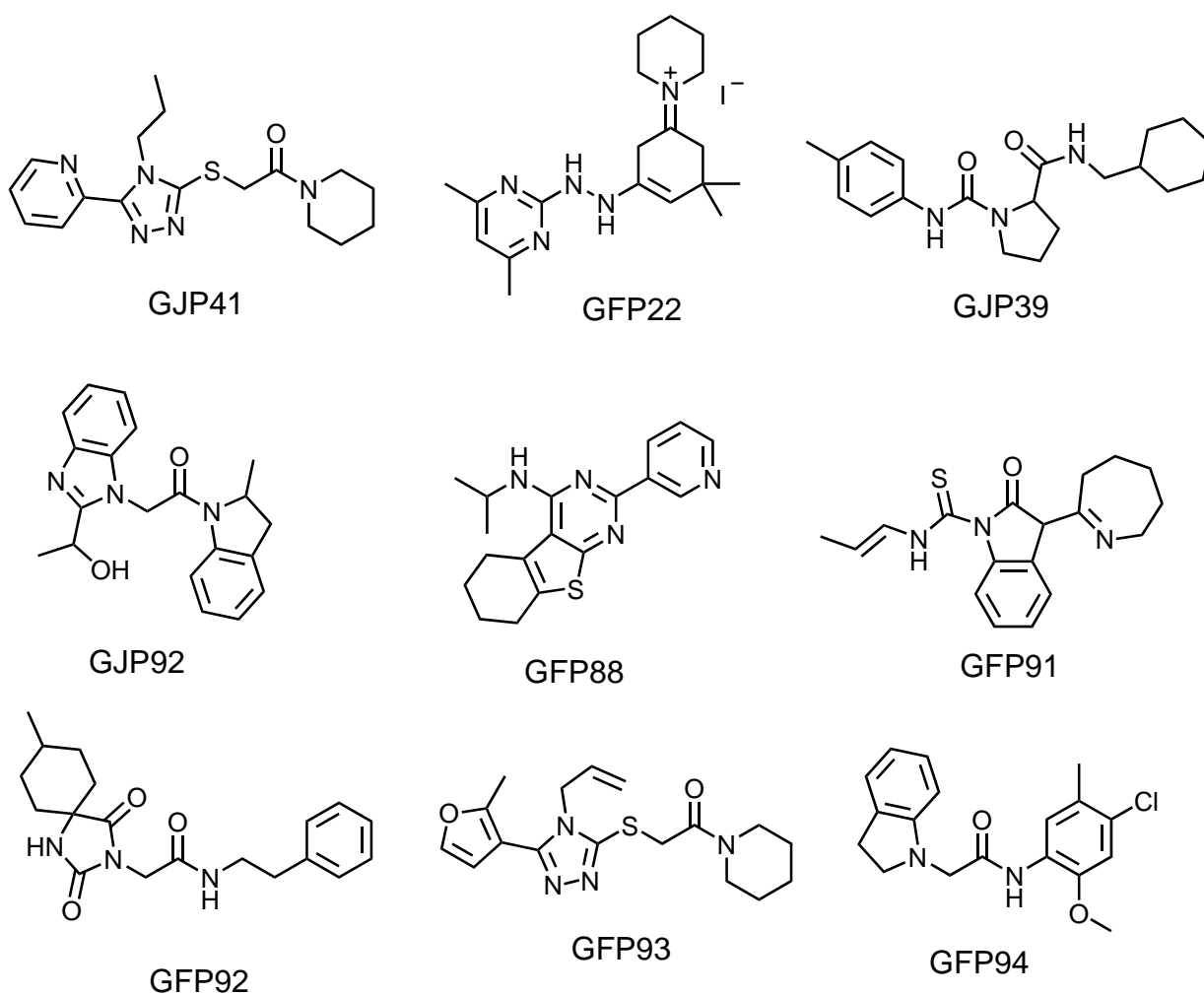
Fig. S3. Chemical structures of GJP41 and GFP22 belonging to category A. Other seven compounds also have increased the levels of PrP Sc in the ex vivo screening.
