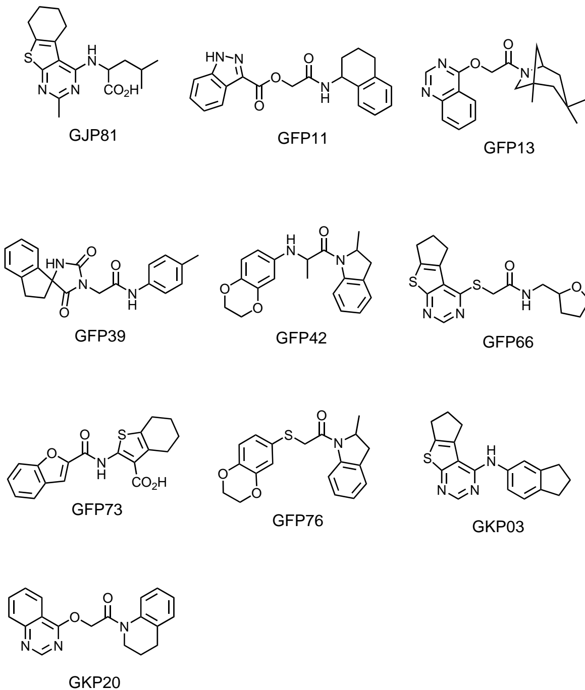
Fig. S1. Chemical structures of compounds belonging to category BNE.
