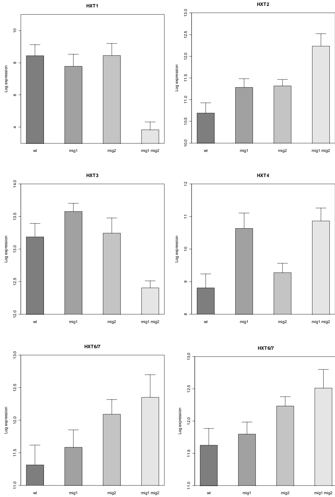
Figure S1: Microarray data for hexose transporters
