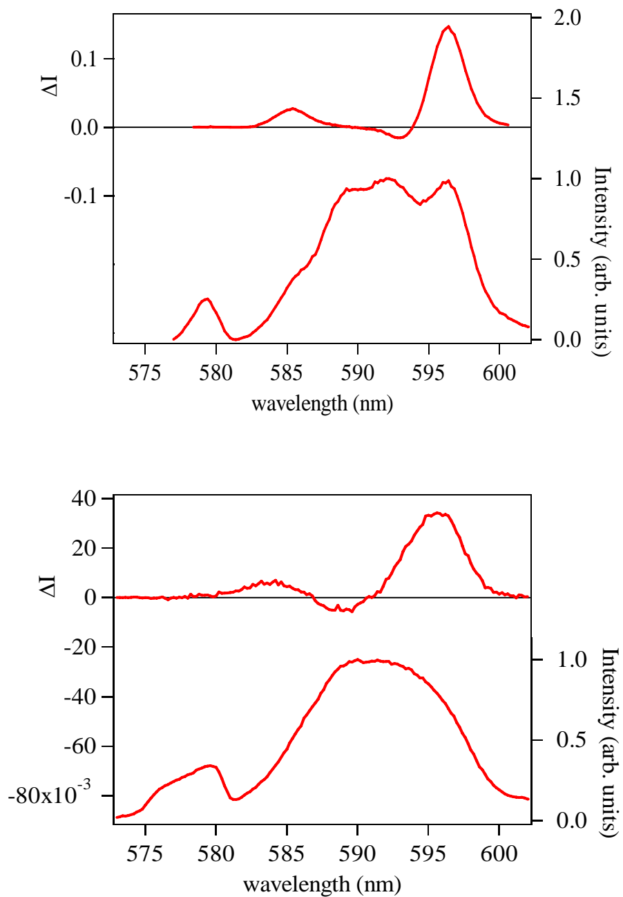
Figure S1 - A comparison of observed CPL behavior for the [EuR(+)BnMeH22IAM] - complex (10 -3 M) with MeOH (top graph) or DMF (lower graph) as solvent. The lower curves in each graph are the observed total luminescence while the upper curves are the observed CPL spectra.
