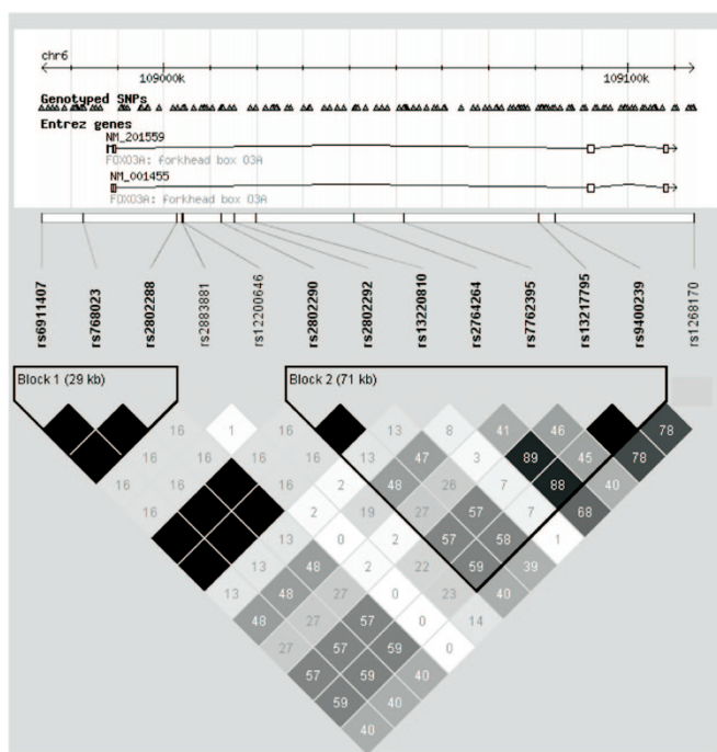
Fig. S1. LD structure of the FOXO3A gene (SNPs genotyped in the German, Dutch, and Japanese samples) according to JPT (A) and CEU HapMap (B) data.
