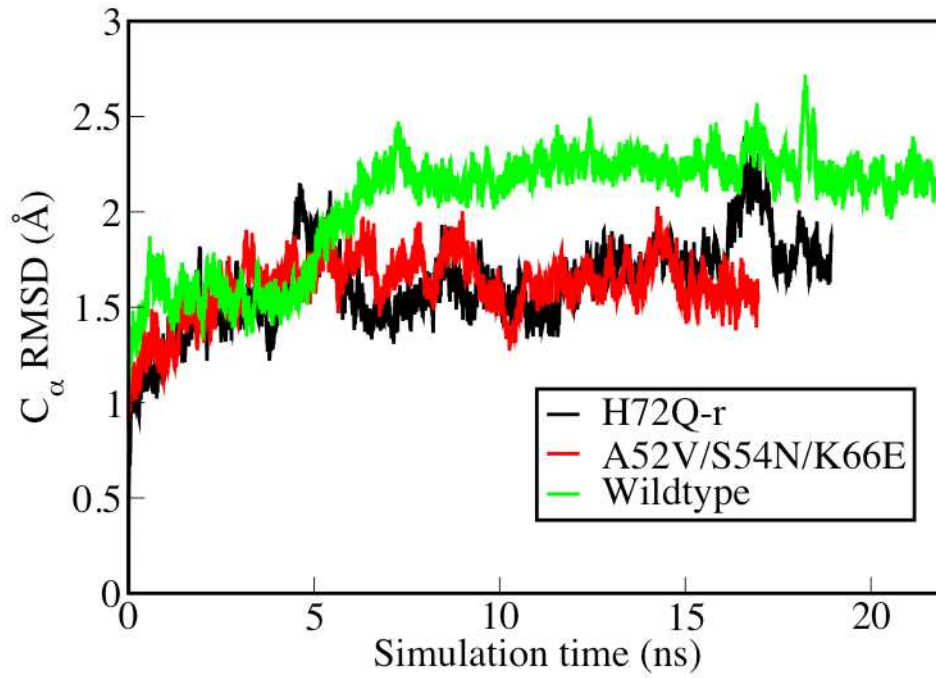
Figure S1. C_{\alpha} RMSD trajectories for the three MD simulations reported.
