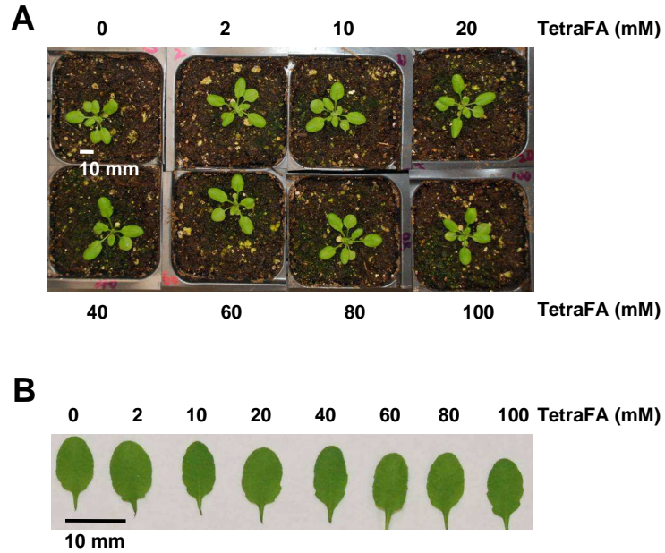
Figure S1. Application of tetraFA from 2 mM - 100 mM to Arabidopsis leaves did not have detectable toxic effect. A and B . Photographs of tetraFA-treated Arabidopsis ( A ) and representative distal leaves ( B ) at 6 dpi. After 1° infection with avirulent Psm AvrRpt2, 10 mM HEPES buffer (pH 7.0) with 0 mM, 2 mM, 10 mM, 20 mM, 60 mM, 80 mM and 100 mM tetraFA was applied to distal leaves by repeated spraying at 3, 24 and 48 hpi.
