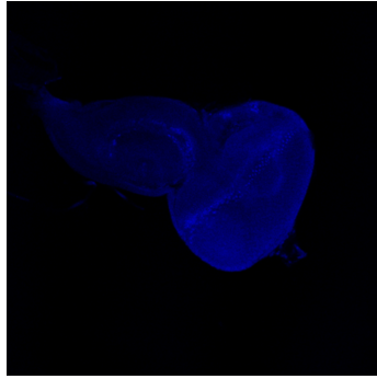
Supplementary Figure 3: Ato, dap and pJNK expression in WT eye discs. Expression of ato in wildtype flies, upregulates Dap and phosphorylated JNK. Third instar eye disc from eyeless-Gal4/UAS-ato
