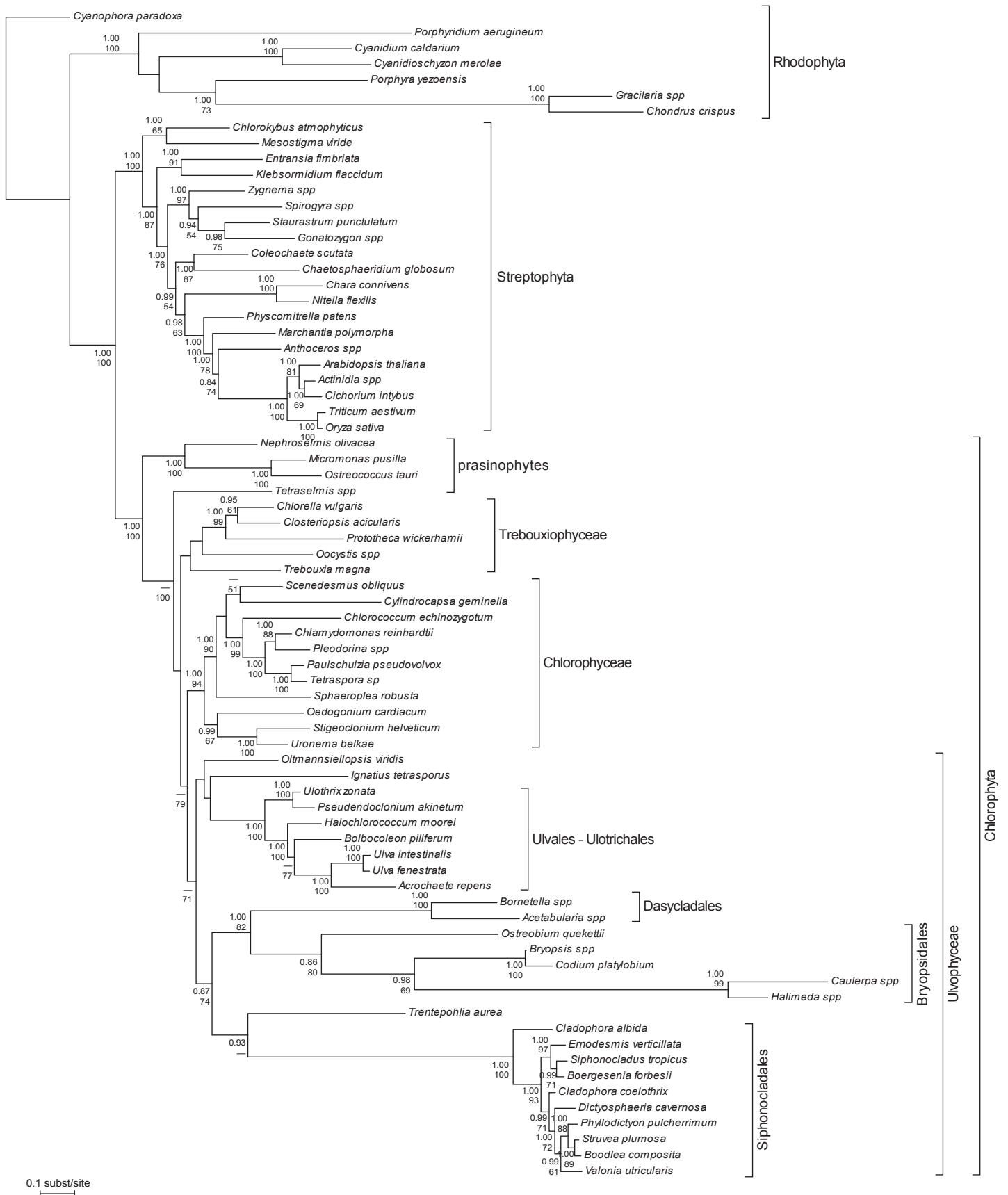
Figure S1. Reference phylogeny of the green plant lineage obtained by Bayesian inference of nuclear SSU rDNA and the plastid genes rbcl and atpB . Numbers at nodes indicate posterior probabilities (top) and ML bootstrap values (bottom); values below respectively 0.9 and 50 are not shown.
