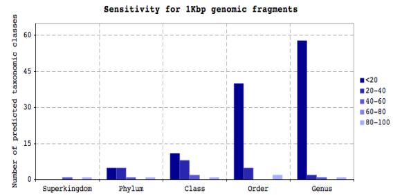
Additional figure 5: Intervals for specificity (left) and sensitivity (right) of predicted taxonomic classes for reads. Classification accuracy intervals for genomic fragments of length 800bp (top) and 1Kbp (bottom). The distribution of number of predicted taxonomic classes at each interval and per taxonomic rank is shown.
