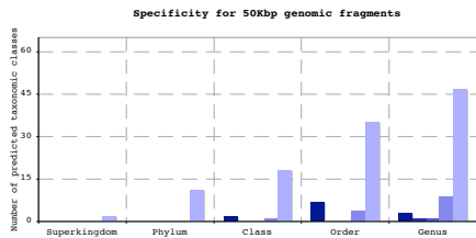
Additional figure 6: Intervals for specificity (left) and sensitivity (right) of predicted taxonomic classes for contigs. Classification accuracy intervals for genomic fragments of length 3Kbp, 10Kbp, 15Kbp, and 50Kbp (from top to bottom). The distribution of number of predicted taxonomic classes at each interval and per taxonomic rank is shown.
