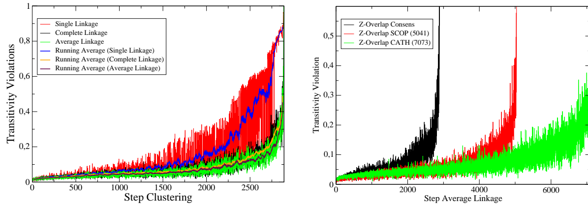
Left plot: Transitivity violations for the single linkage, average linkage and complete linkage algorithms. Right plot: Transitivity violations for three sets of domains with 2890, 5041 and 7073 domains respectively.
