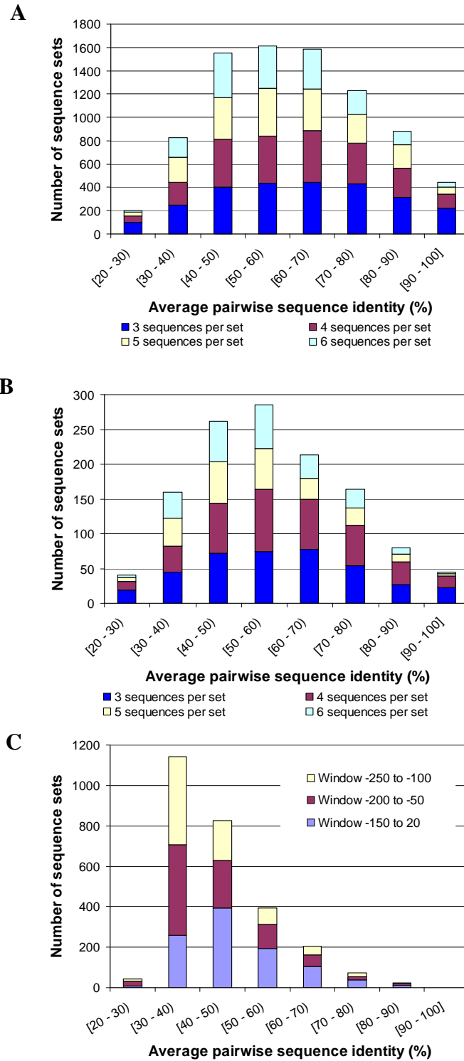
Figure S4. Distribution of sequence identities and size of the sequence sets studied. A. Training sets. B. Test sets. C. Shewanella sequence sets.
