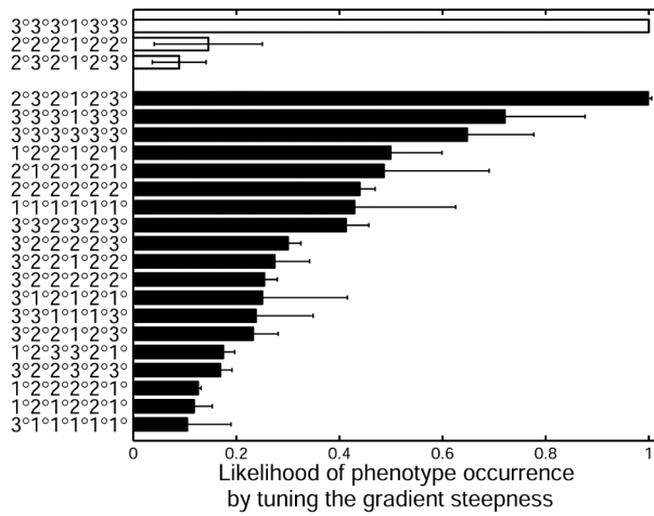
Figure S3. Phenotypic diversity caused by quantitative changes in gradient steepness. Mutant phenotypes with greatest likelihood of phenotype occurrence upon an increase (empty) and decrease (filled) in the steepness of the gradient in inductive signal ( \Delta I ).
