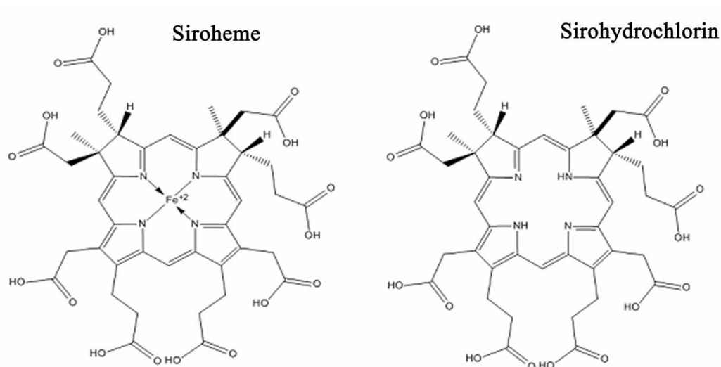
Figure S1 – Schematic representation of the siroheme and sirohydrochlorin molecules. Images generated in ChemBioDraw – version 11.0.1, CambridgeSoft – Life Science Enterprise Solutions.
