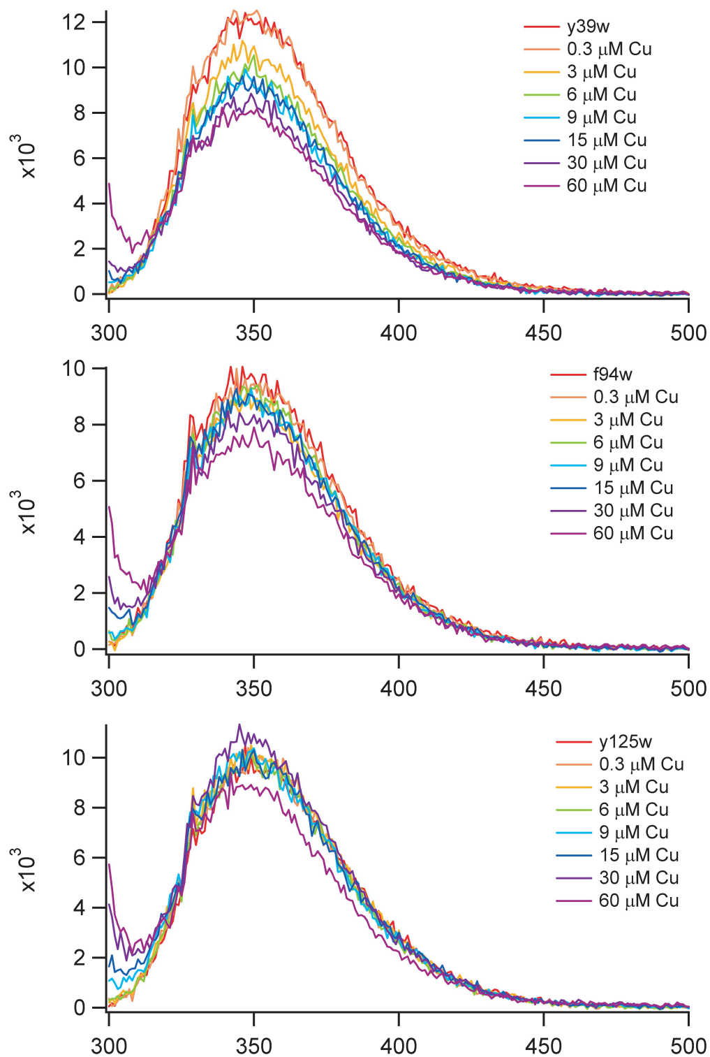
Figure2S. Fluorescence of Trp-containing synuclein as a function of Cu(II) added. [protein]=1.6-2 \mu\text{M} , in 20 mM MOPS, 100 mM NaCl, pH 7. Excited at 295 nm.
