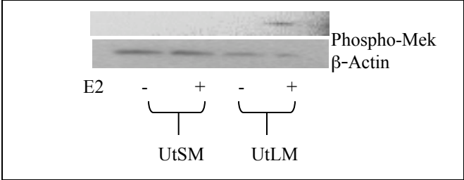
Figure 6. Phospho-Mek levels with E2 treatment.
