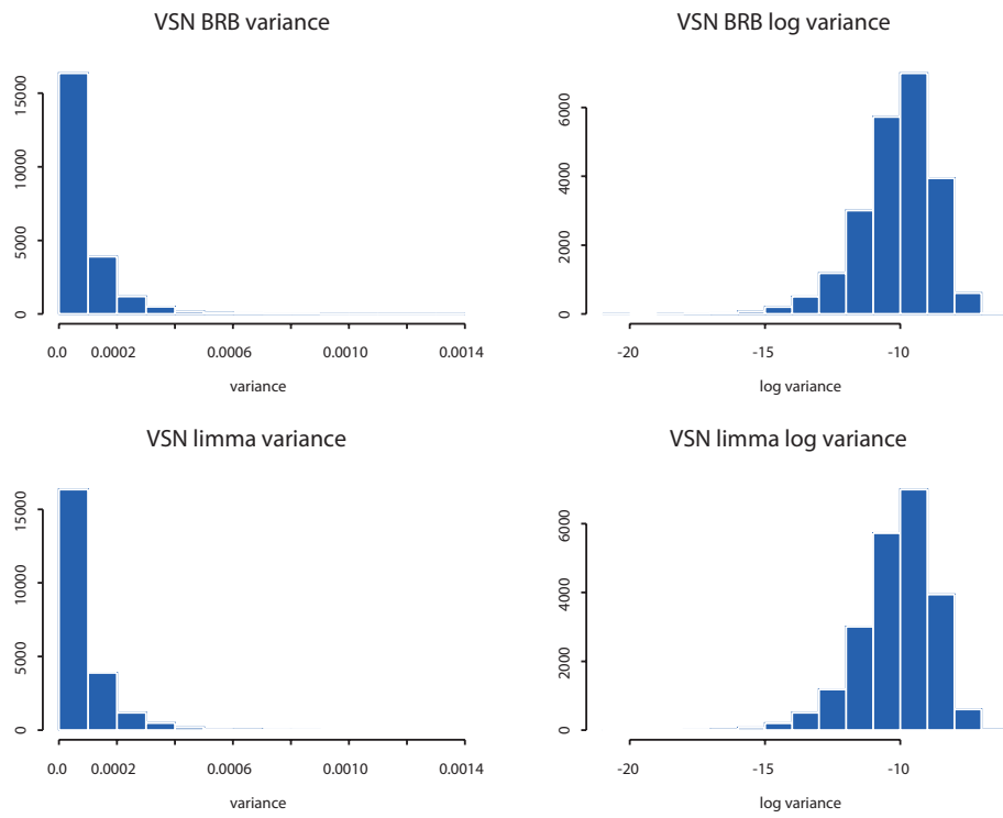
Figure 2: Histograms of posterior variances, logged and unlogged, for BRB and limma statistical tests using VSN normalized data.
