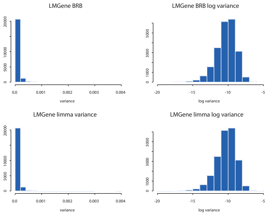
Figure 1: Histograms of posterior variances, logged and unlogged, for BRB and limma statistical tests using lmGene normalized data.
