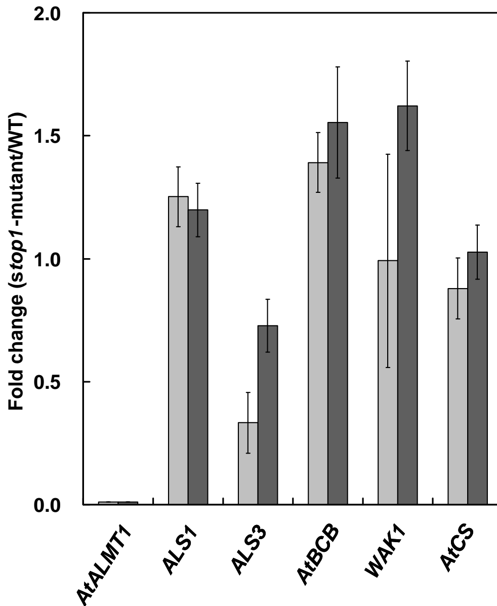
Supplemental Figure S1. Fold change of gene expression in microarray, whose gene is associated with Al tolerance as follows; AtALMT1 (Hoekenga et al., 2006), ALS1 (Larsen et al., 2007), ALS3 (Larsen et al., 2005), AtBCB (Ezaki et al., 2000), WAK1 (Sivaguru et al., 2003), AtCS (Koyama et al., 2000). Biologically independent 3 replication of competitive microarray analyses were carried out as follows; stop1 -mutant versus wild type in Al (10 μM, 24 h; light gray) and low pH (pH 4.5, 24 h; dark gray). Fold change and whose \pm SD are shown.
