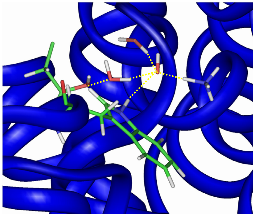
Figure S1. A snapshot showing the hydrogen bonding interactions of the hydroxide anion with surrounding residues and solvent molecules at the transition state in the deprotonation of ammonium cation.
