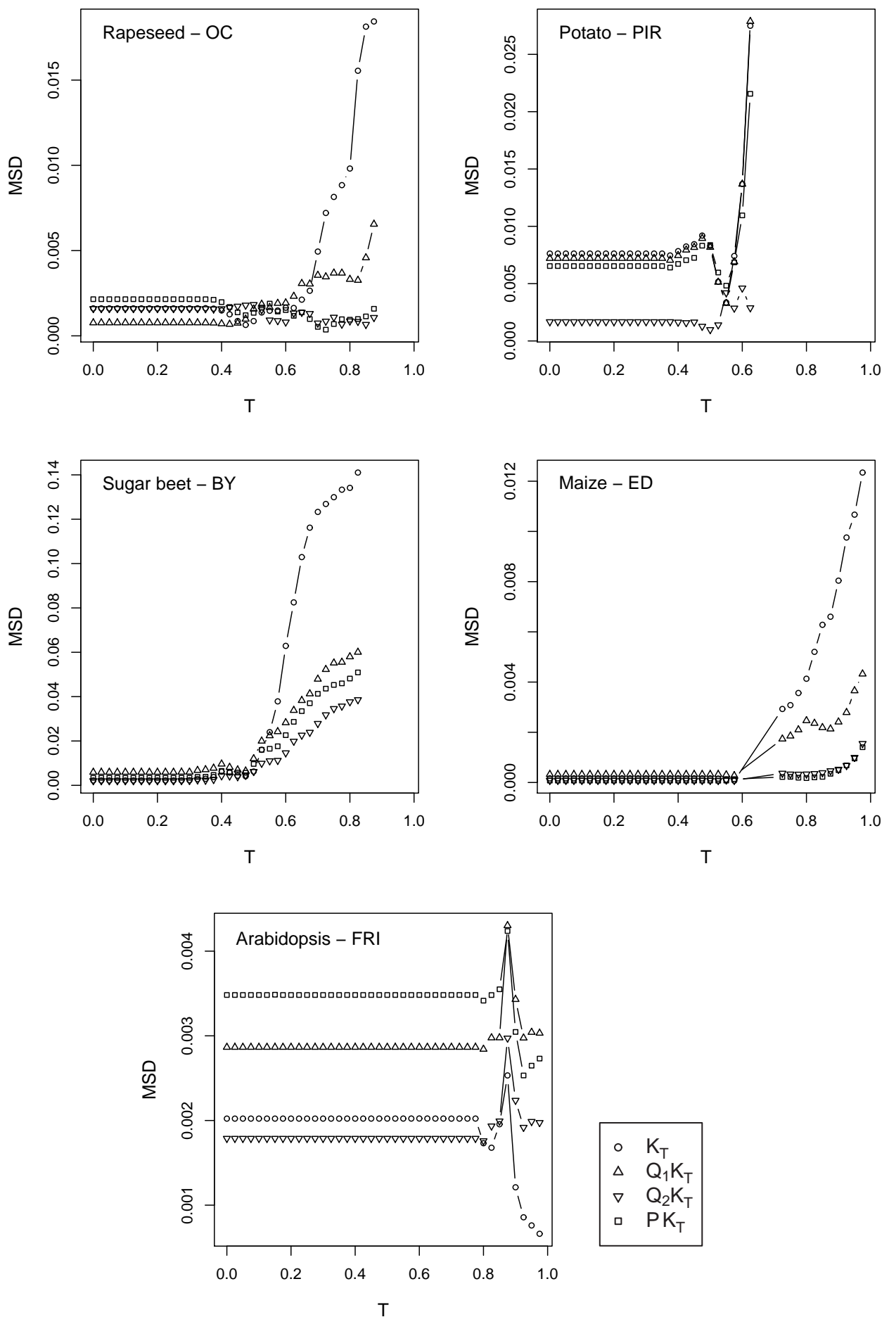
Additional file 3. Mean of squared differences (MSD) between observed and expected P values for four different mixed-model association mapping methods depending on threshold T . For each of the five plant species, the result of the trait with medium genetic complexity is presented. The incomplete profiles for rapeseed, potato, and sugarbeet are due to convergence problems for the corresponding T values.
