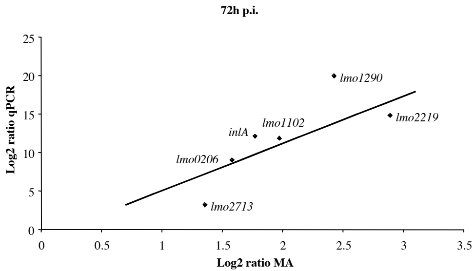
Figure S2: Validation of macroarray data by real-time RT-PCR. Fold changes in in vivo gene expression 24h p.i. (A) or 72h p.I. (B) compared to that in BHI were measured by macroarray and real-time RT-PCR, log transformed and compared for correlation analysis.
