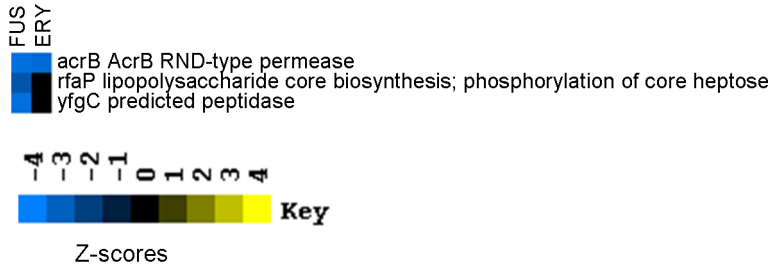
Figure S7. Loci whose disruption was significant in at least one inhibitor of the 50S subunit of the ribosome. Yellow (blue) indicates that transposon insertions in or near a gene were beneficial (deleterious). Black indicates no significant effect. Z-scores were calculated as described in Materials and Methods .
