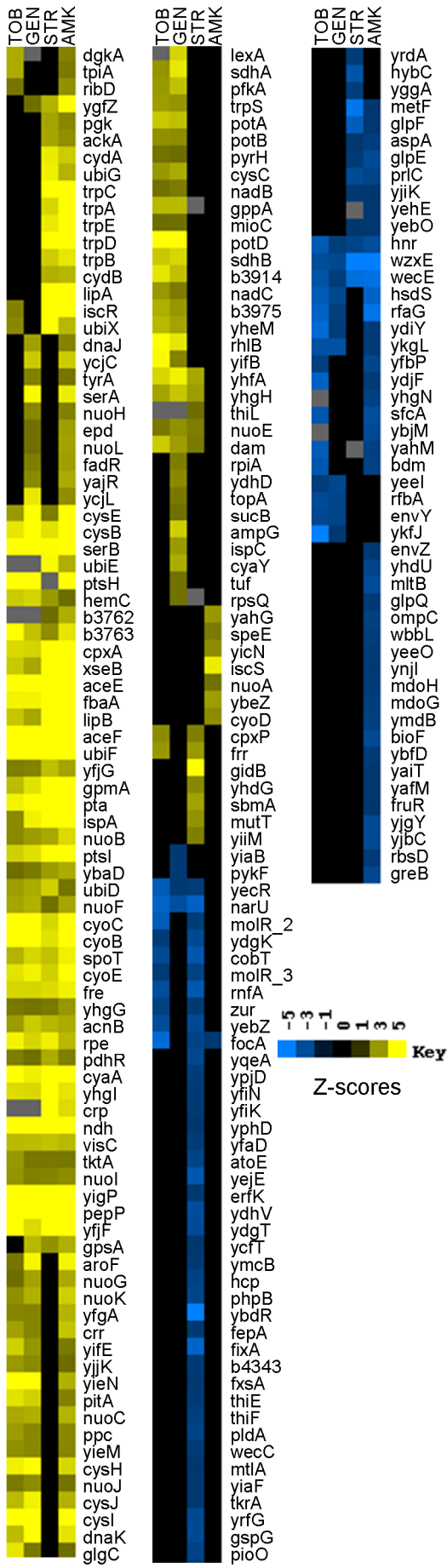
Figure S11. Loci whose disruption was significant in at least one aminoglycoside.
