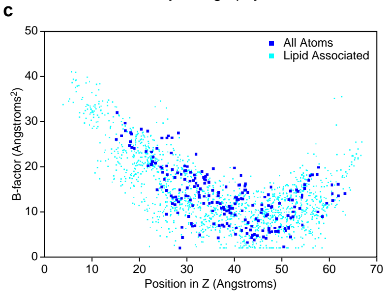
Electron Crystallography Structure
