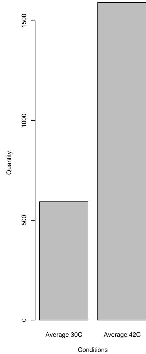
SCO4410
