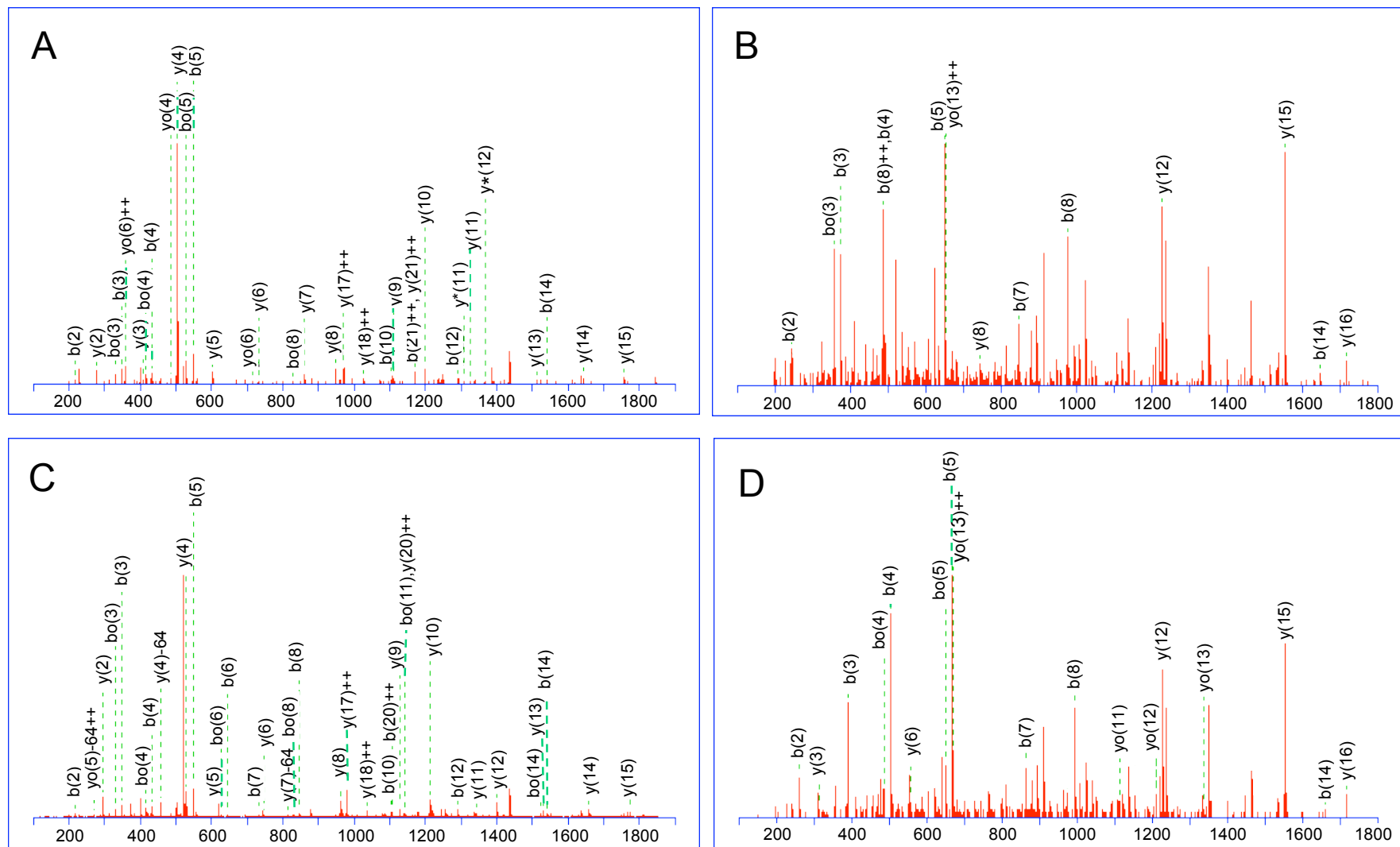
Supplemental Fig. 2. Q-TOF MS/MS spectra for endogenous PENK 239-260 (A) and PENK 114-133 (B), and synthetic PENK 239-260 (C) and PENK 114-133 (D).
