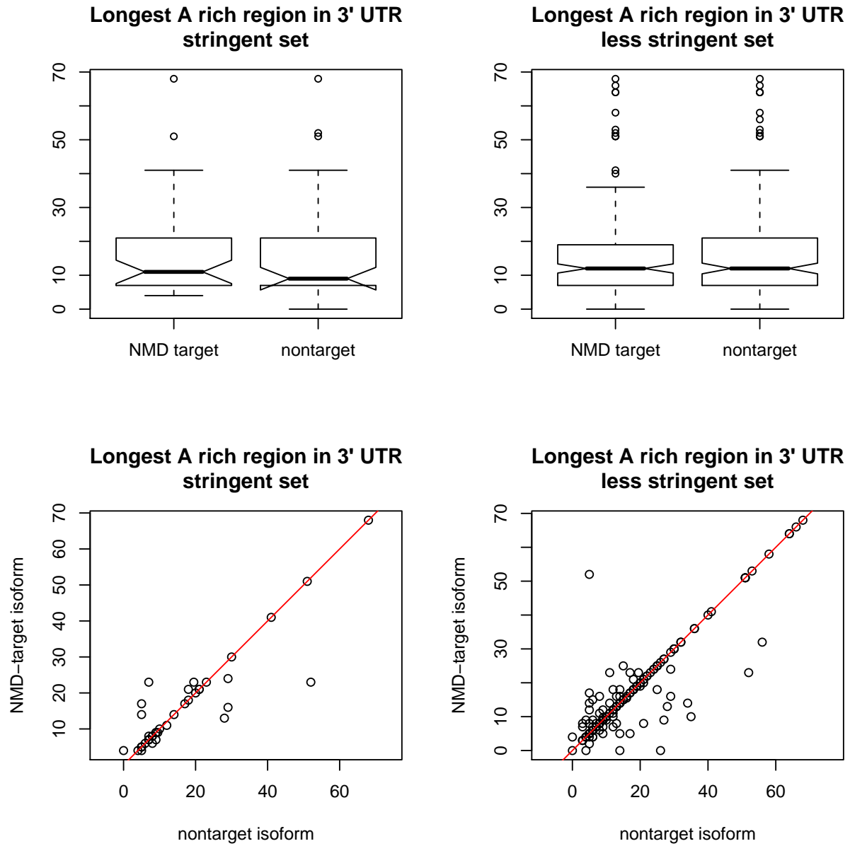
Figure S17. Length of longest A-rich region in 3' UTR. As Figure S9 for the feature “length of longest A-rich region in 3' UTR.”
