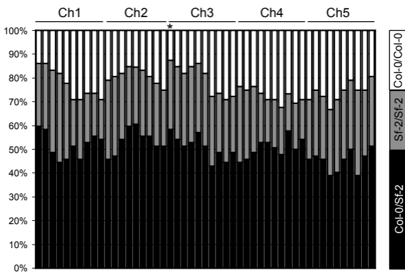
Supplemental Figure 1. Genotype segregation of Sf-2 x Col-0 F2 progeny at each marker position. The fit to the expected F2 segregation ratio (1:2:1) was analyzed using a G-test (*: 0.01 < P < 0.05 ). The column to the right of the bar graph represents the expected segregation, 50% of heterozygote and 25% of each homozygote.
