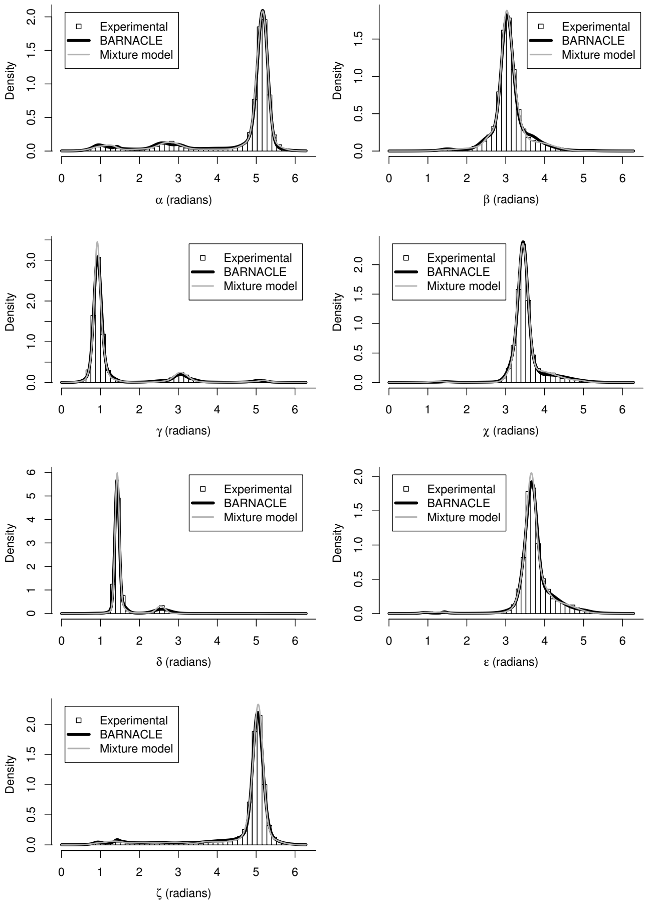
Figure S1. The marginal distributions of all seven individual angles. The distributions in the experimental data set are shown as histograms. The density functions for the mixture model are shown as gray lines. The black lines show the densities for BARNACLE, calculated from the stationary probability distributions [Cappé O, Moulines E, Ryden T (2005) Inference in hidden Markov models. New York: Springer. 654 p.].
