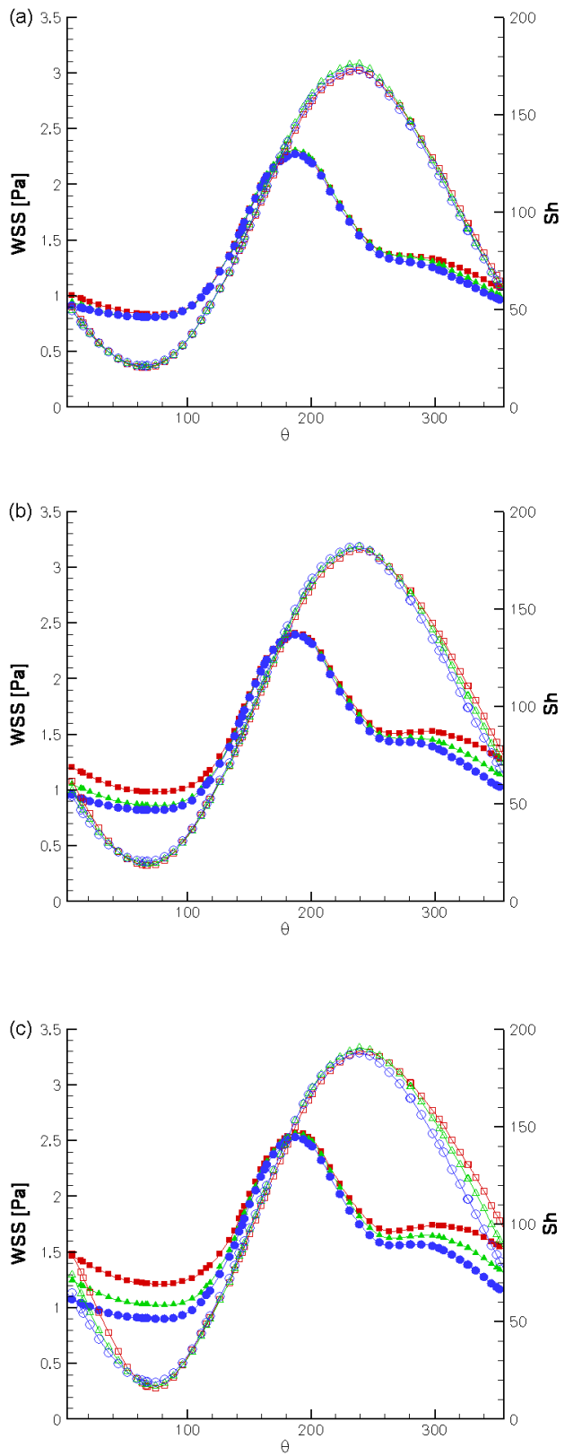
Figure 13. Time-averaged WSS (filled symbols) and Sh (open symbols) number profiles along the circumference of the proximal section and (a) A=0.66 , (b) A=1 and (c) A=1.33 . Squares, T=0.5 s; triangles, T=0.8 s; circles, T=1.33 s.
