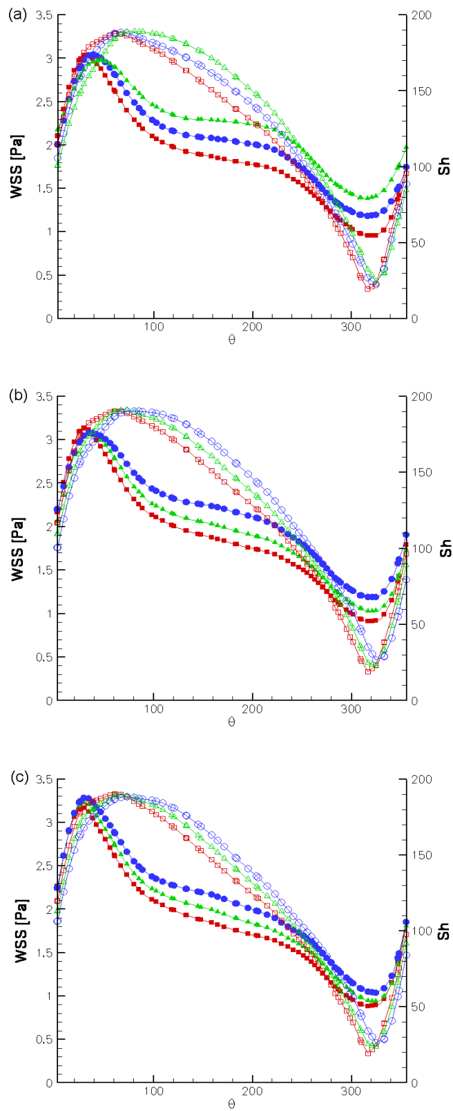
Figure 14. Time-averaged WSS (filled symbols) and Sh (open symbols) number profiles along the circumference of the middle section and (a) T=0.5 s, (b) T=0.8 s and (c) T=1.33 s. Squares, A=0.66 ; triangles, A=1 ; circles, A=1.33 .
