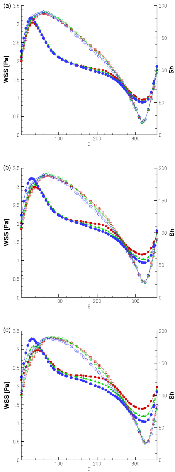
Figure 15 Time-averaged WSS (filled symbols) and Sh (open symbols) number profiles along the circumference of the middle section and (a) A=0.66 , (b) A=1 and (c) A=1.33 . Squares, T=0.5 s; triangles, T=0.8 s; circles, T=1.33 s.
