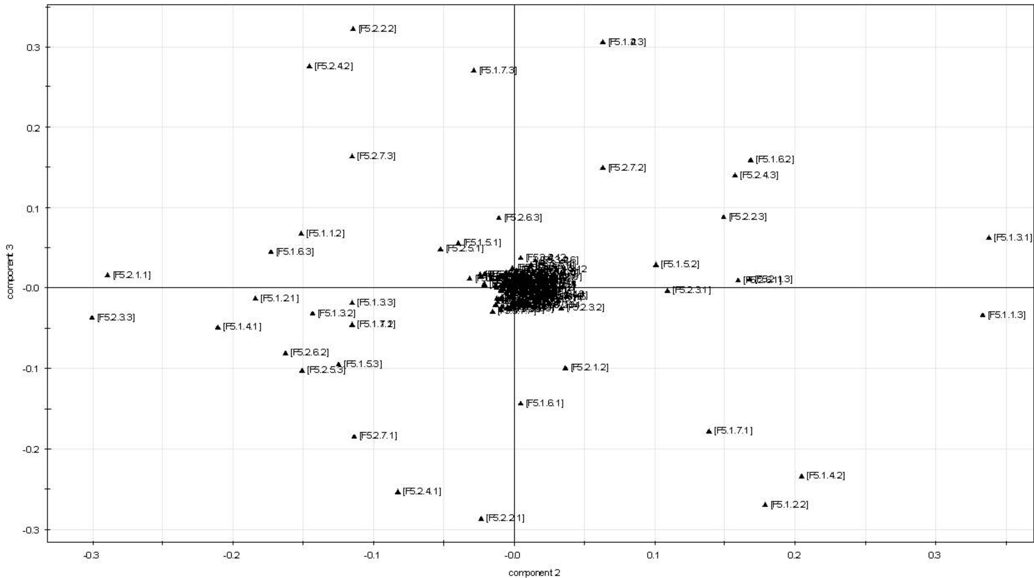
Protein Descriptors component 2 vs. component 3
