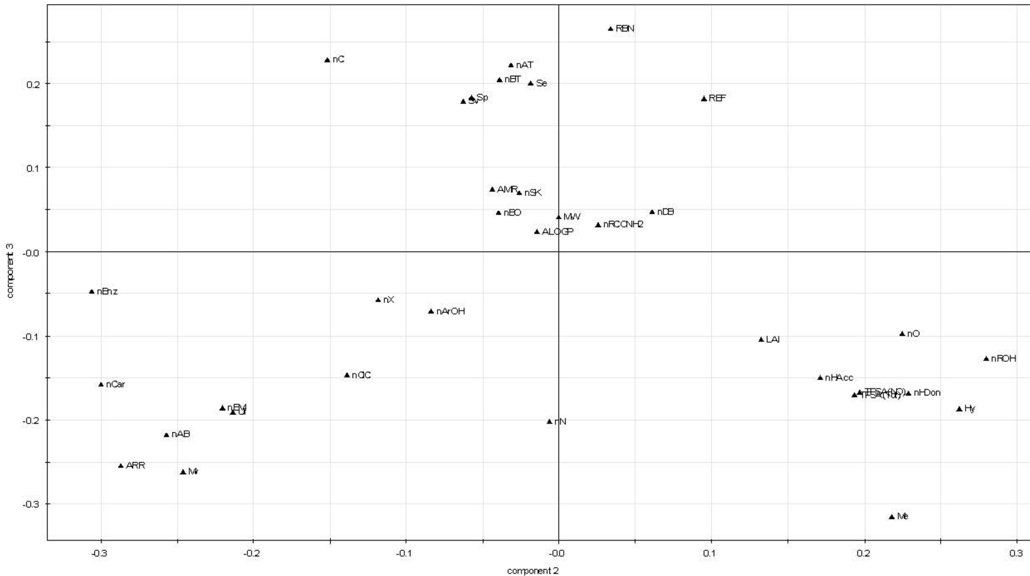
Ligand Descriptors component 2 vs. component 3
