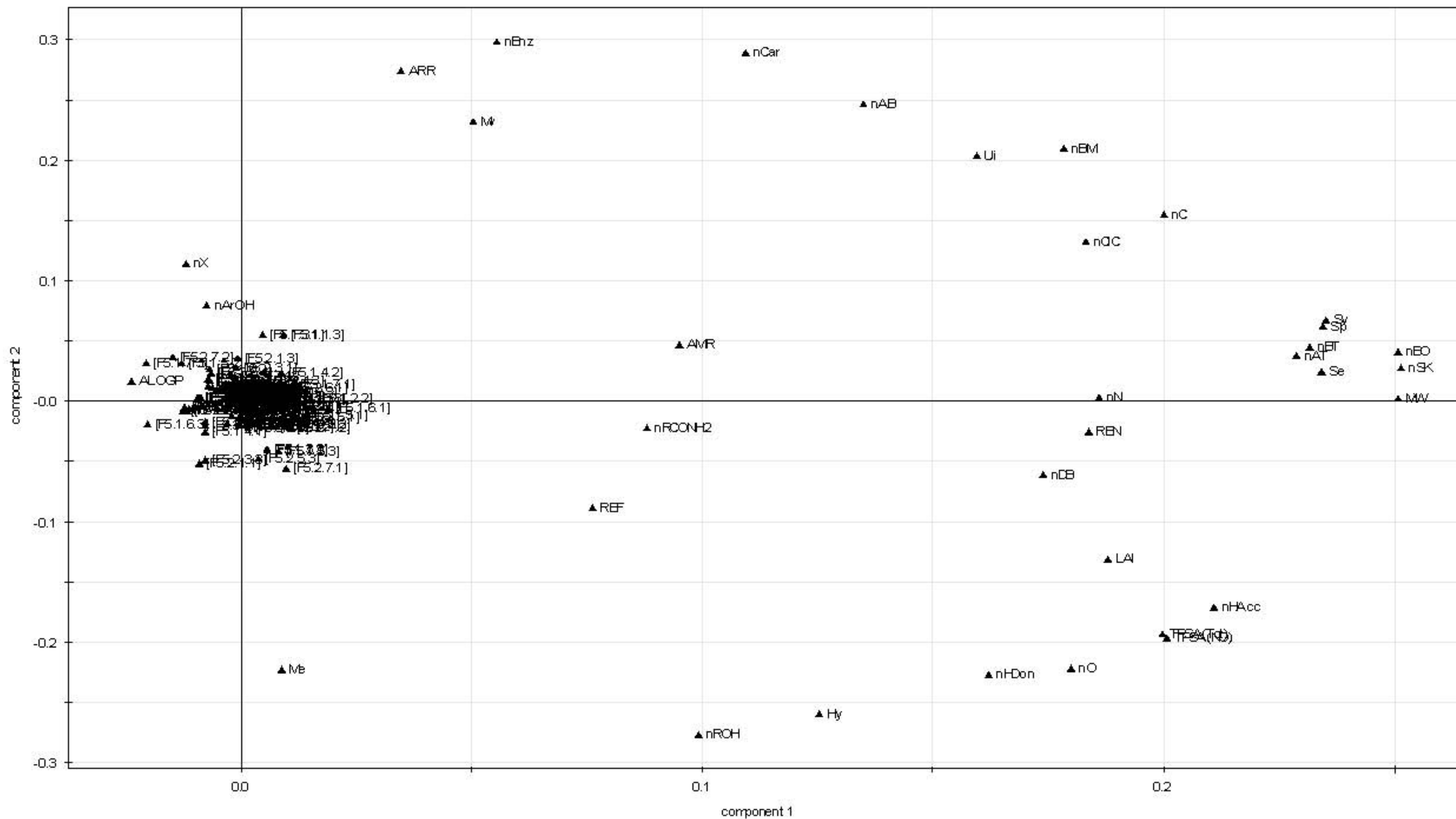
Protein and Ligand Descriptors component 1 vs. component 2
