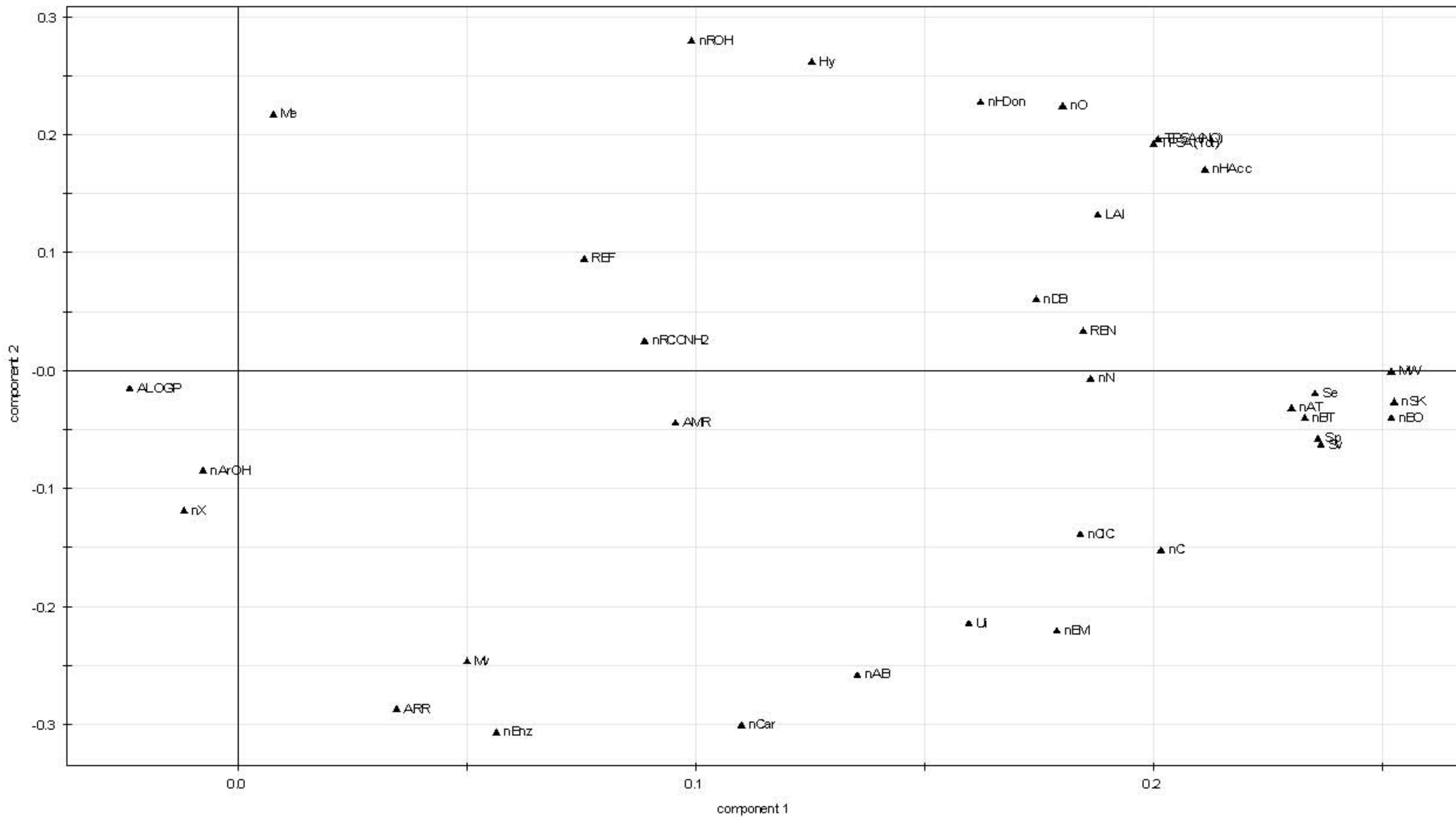
Ligand Descriptors component 1 vs. component 2
