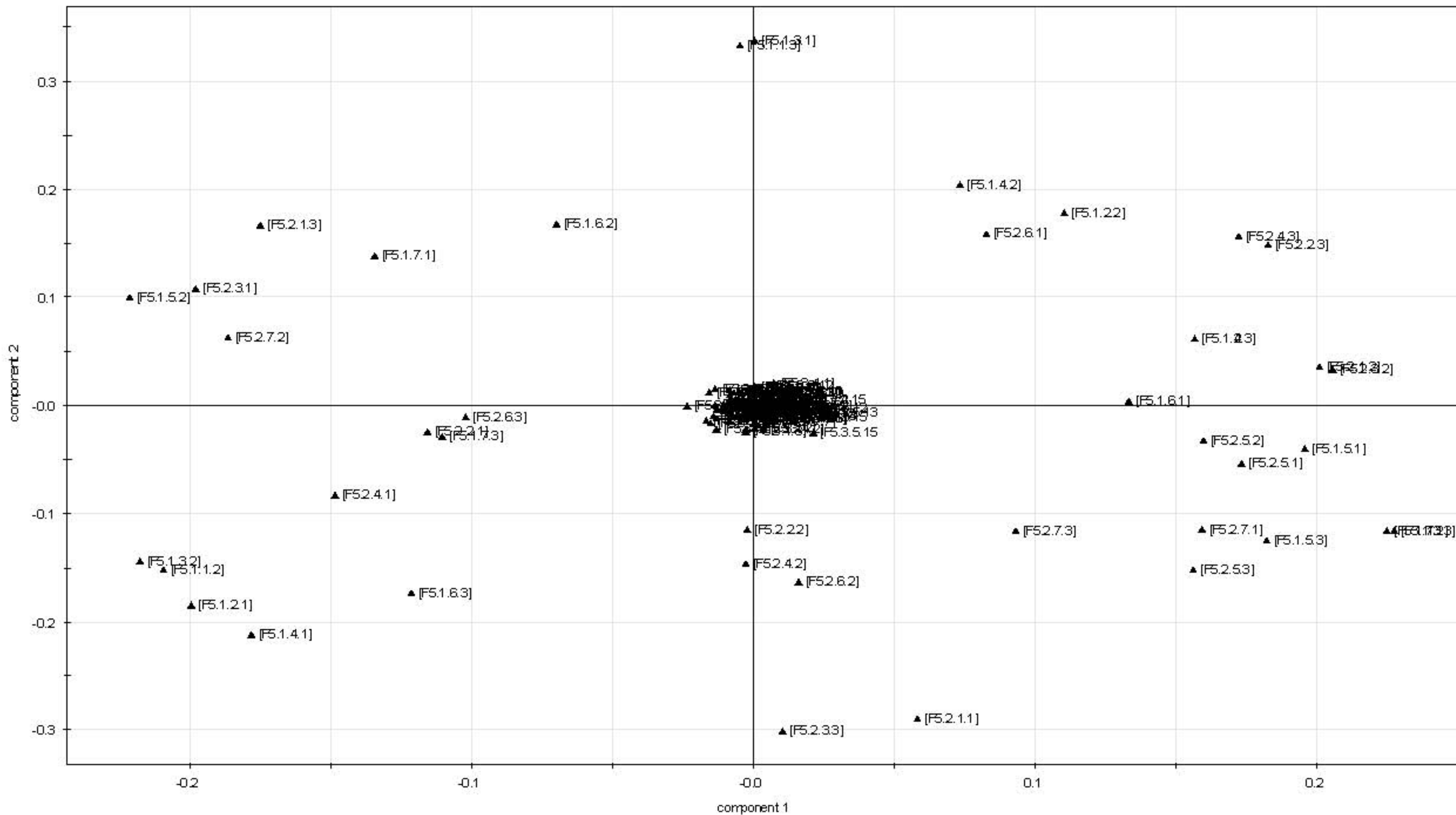
Protein Descriptors component 1 vs. component 2
