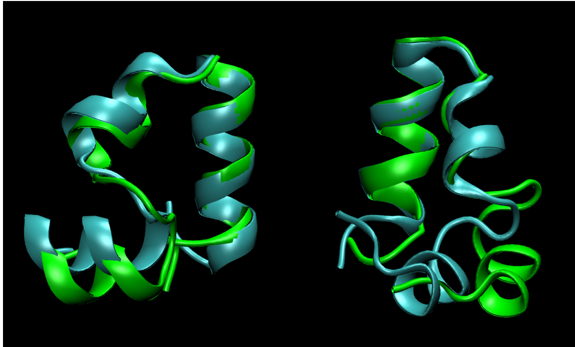
Figure S1 Fluctuation of helix I in experimental structures. Left: superposition of the X-ray structure (cyan, PDB code 1YRF) and average NMR structure (green, PDB code 1VII). Right: superposition of two NMR structures (courtesy of C.J. McKnight). For clarity, the structures are in different orientations than in Figure 4.
