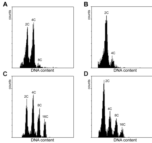
Figure S1. Effect of co-expression of CYCA2;3-nGFP and CDKB1;1-cGFP . Col-0 seedlings (A and C) and plants co-expressing CYCA2;3-nGFP and CDKB1;1-cGFP (B and D) were grown for 12 DAG on agar medium and 1 st leaf pairs and roots were harvested. Leafs (A and B) and roots (C and D) were subjected to flow cytometry (C and D).
