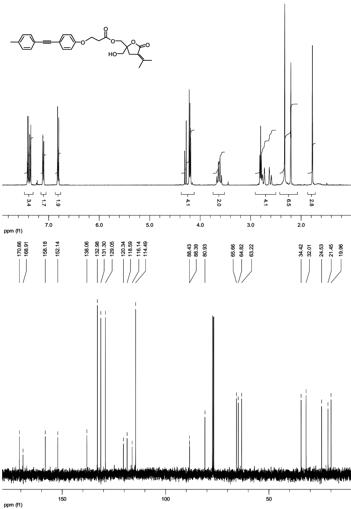
1 H and 13 C spectra of 1b .
