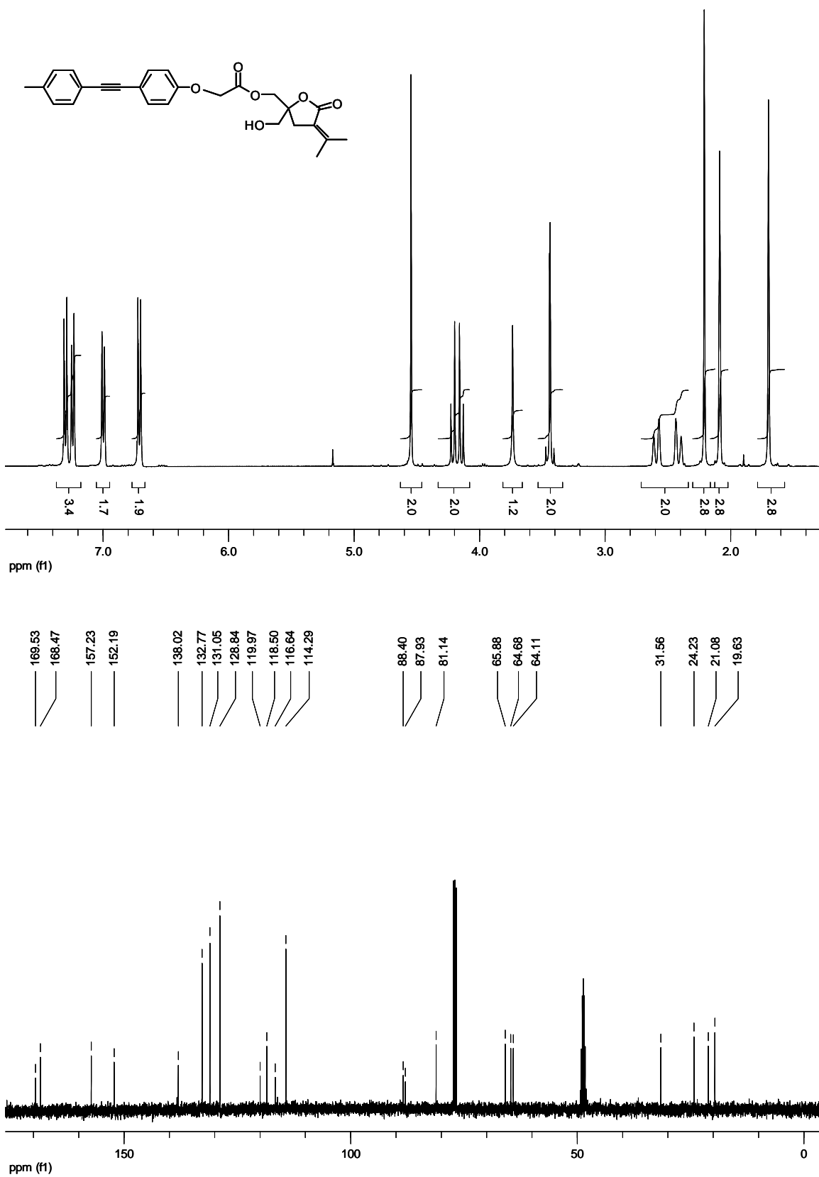
1 H and 13 C spectra of 1a .
