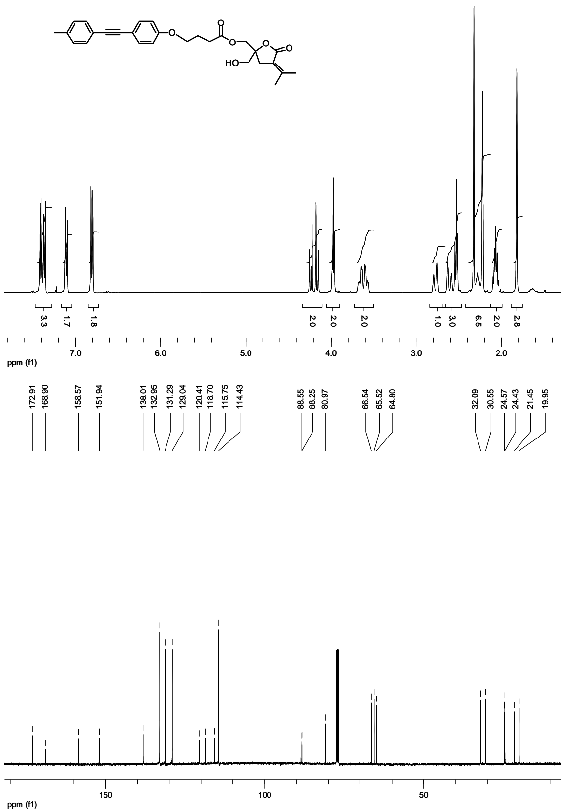
1 H and 13 C spectra of 1c .
