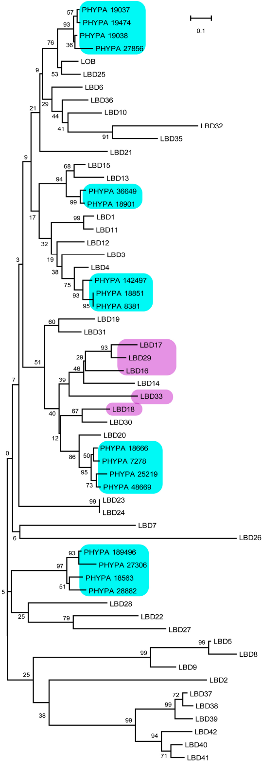
File 13. Phylogenetic relationship (neighbor-joining (NJ) method) of A. thaliana and P. patens LBD proteins.
