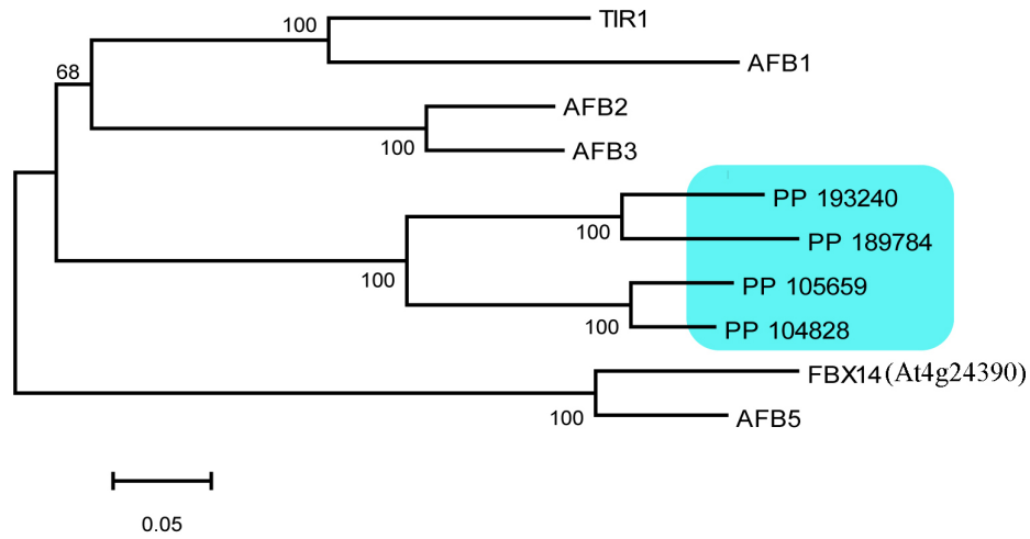
File 4. Phylogenetic relationship of A. thaliana and P. patens TIR1-like F-box proteins (Neighbor Joining (NJ) method).
