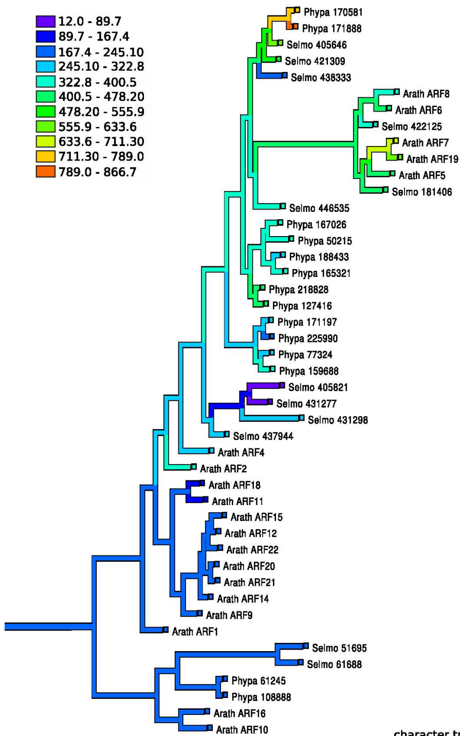
File 8. Phylogenetic relationship of A. thaliana , S. moellendorffii and P. patens ARF proteins (reconciled tree based on Bayesian inference). Length of middle region was normalized and transformed into a continuous character matrix.
