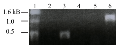
Figure S2. KP strain 43816 is an aerobactin negative strain. KP lysates underwent PCR analysis for aerobactin (500 bp amplicon) as described. Lane 1- molecular weight standard, lane 2 – KP ATCC strain 43816, lane 3 – known aerobactin-positive KP strain, lane 4 – known aerobactin-negative KP strain, lane 5 – known aerobactin-negative E. coli strain, lane 6 – positive control for PCR using irrelevant primers and KP 43816 lysate.
