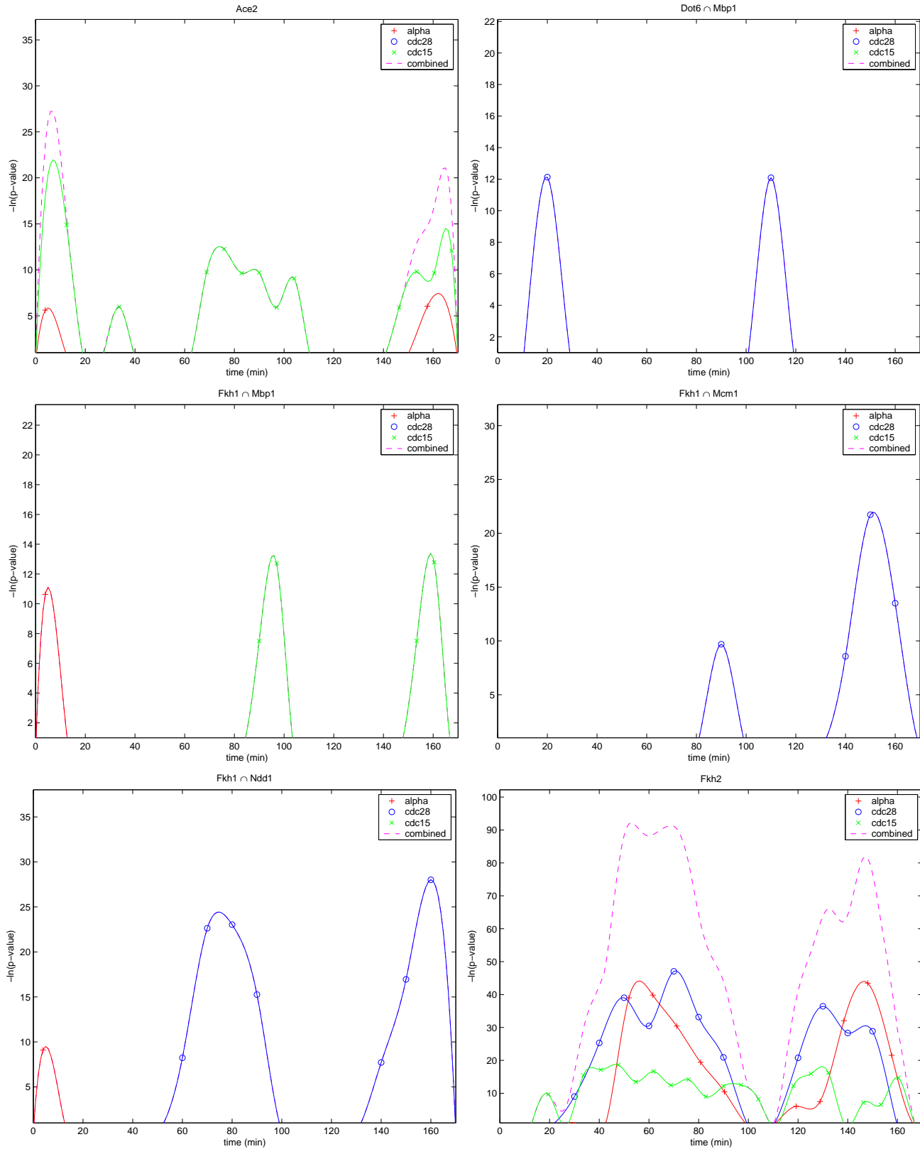
Supplementary Figure 1. Rule profiles that show cell-cycle dependency.
