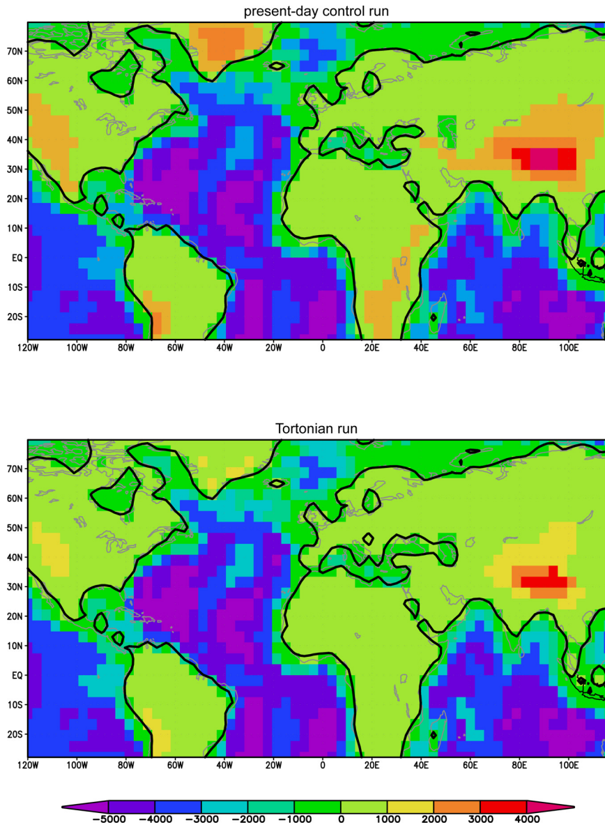
Fig. S3. The land-sea distribution, orography, and bathymetry of the Tortonian and present-day control run.
