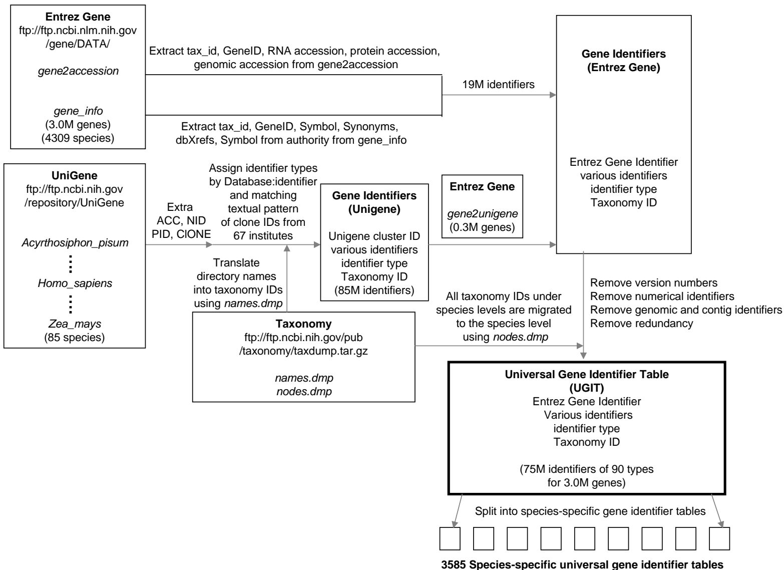
Supplementary Fig. 1: Flow chart diagram illustrating the creation of UGIT from Entrez Gene and UniGene files
